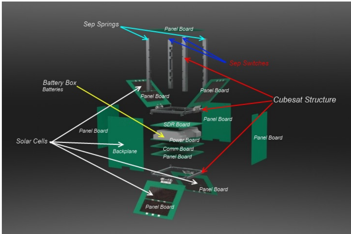
Figure 2: CAPE-2 Expanded View
