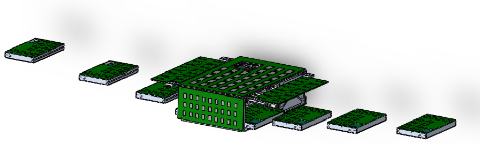
Figure 3: ANDESITE Sensor Node Deployment & Node Expanded View
