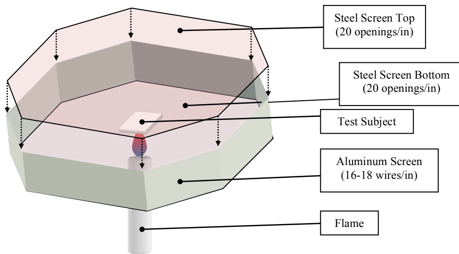
Figure 4: Underwriters Laboratory Explosion Test Apparatus
