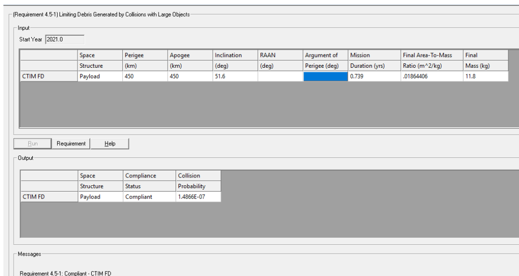
Figure 5 Limiting Debris Generated by Collisions with Large Objects
