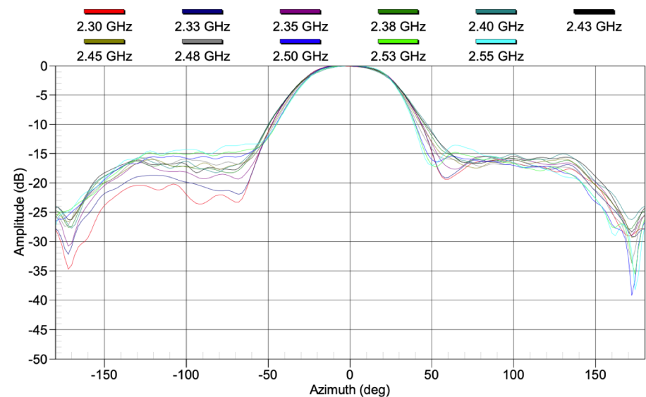
Figure 5: Typical Far Field Pattern - SNT Horizontally Aligned to Horizontally Aligned Horn Antenna
