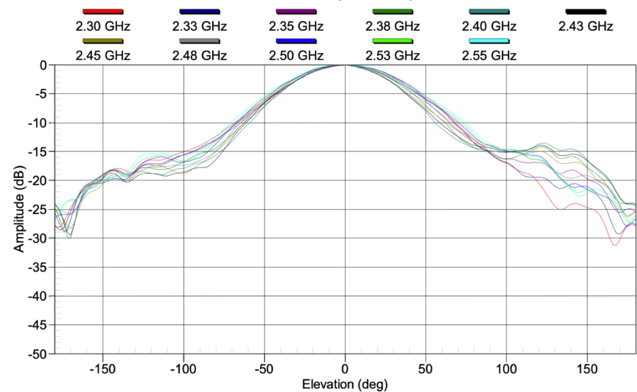
Figure 6: Typical Far Field Pattern - SNT Vertically Aligned to Vertically Aligned Horn Antenna
