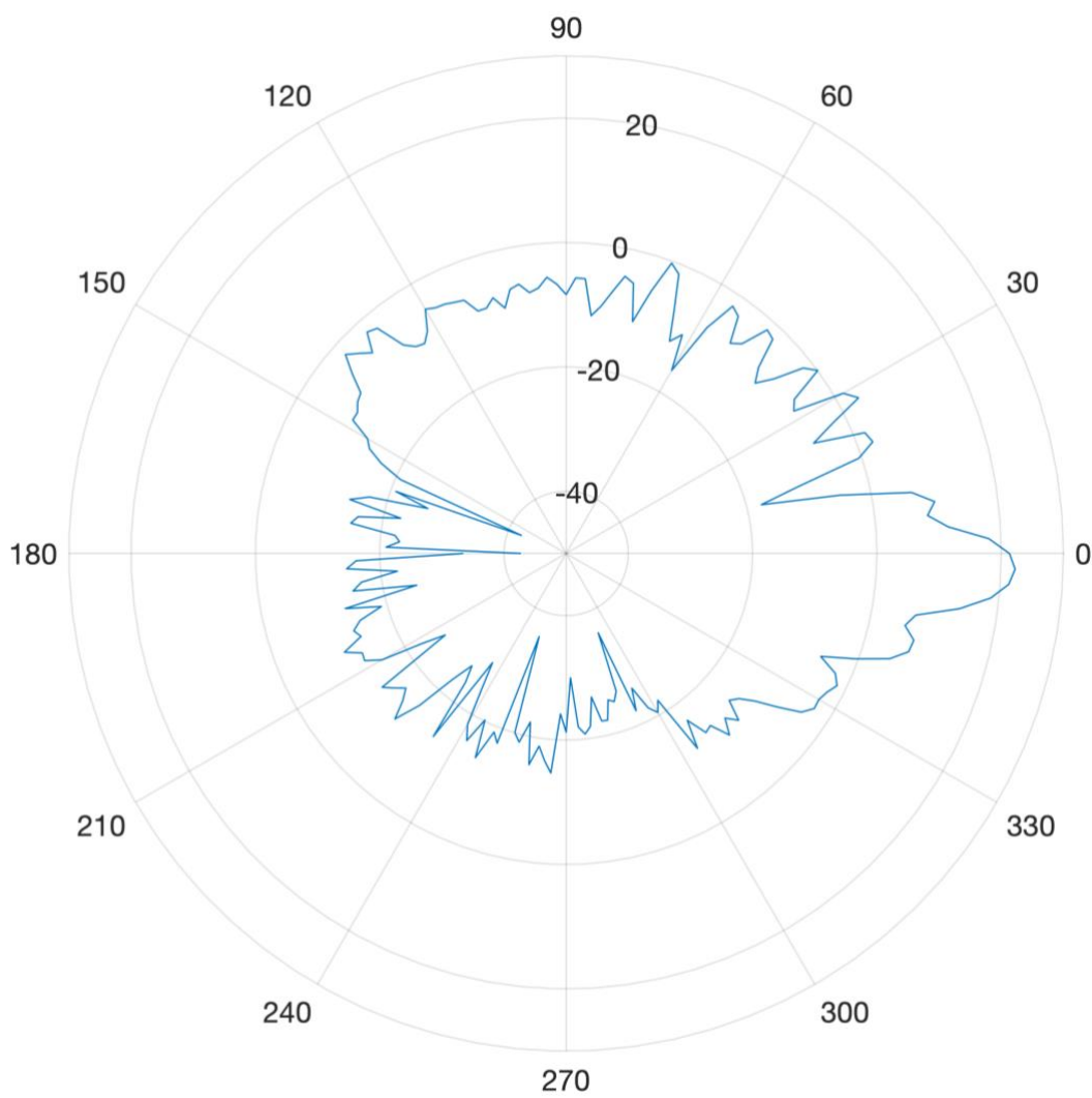
Feedhorn Antenna and Reflectarray Radiation Pattern at 8.45 GHz and \phi = 95^\circ for \theta = 0^\circ to \theta = 360^\circ
