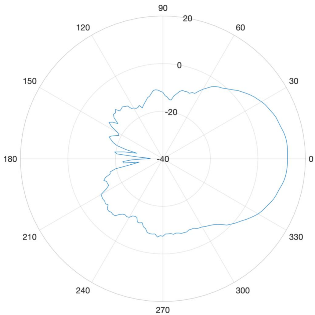
Feedhorn Antenna Radiation Pattern at 8.5 GHz and \phi = 0^\circ for \theta = 0^\circ to \theta = 360^\circ
