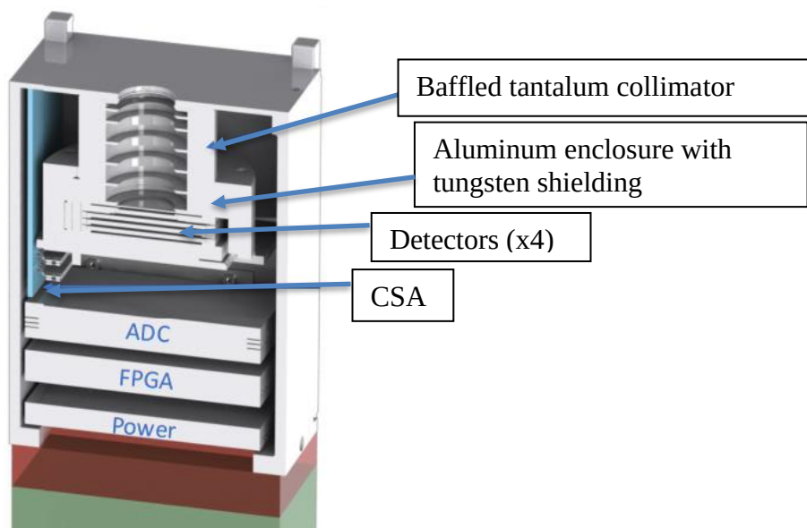
Figure 2, Payload cutaway showing REPTile-2, heavy metal shielding, and associated electronics boards
