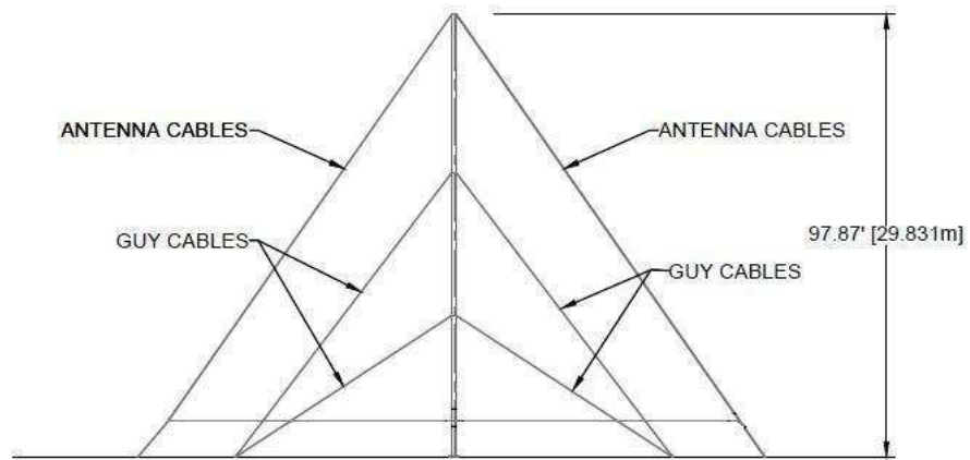
TRANSMIT (TX) TOWER / ANTENNA SIDE VIEW
