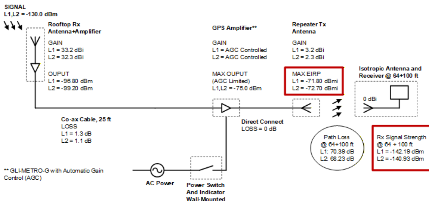
Figure 5 GPS Re-Radiator RF Signal Link Budget Analysis
