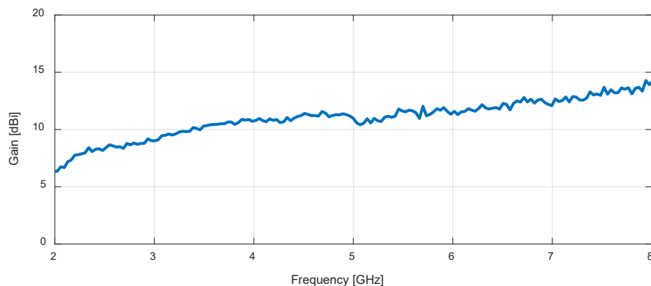
Figure 1 - Measured Antenna Gain at CReSIS Anechoic Chamber
