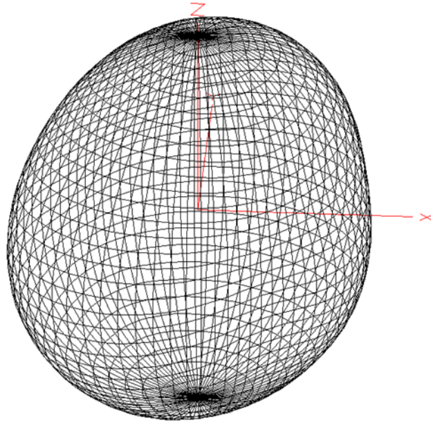
Figure 3: L-Dipole UHF Antenna Gain Plot
