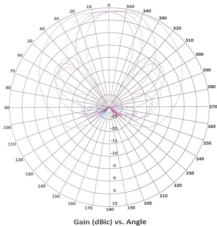
Figure 4: X-band Antenna Gain Plot
