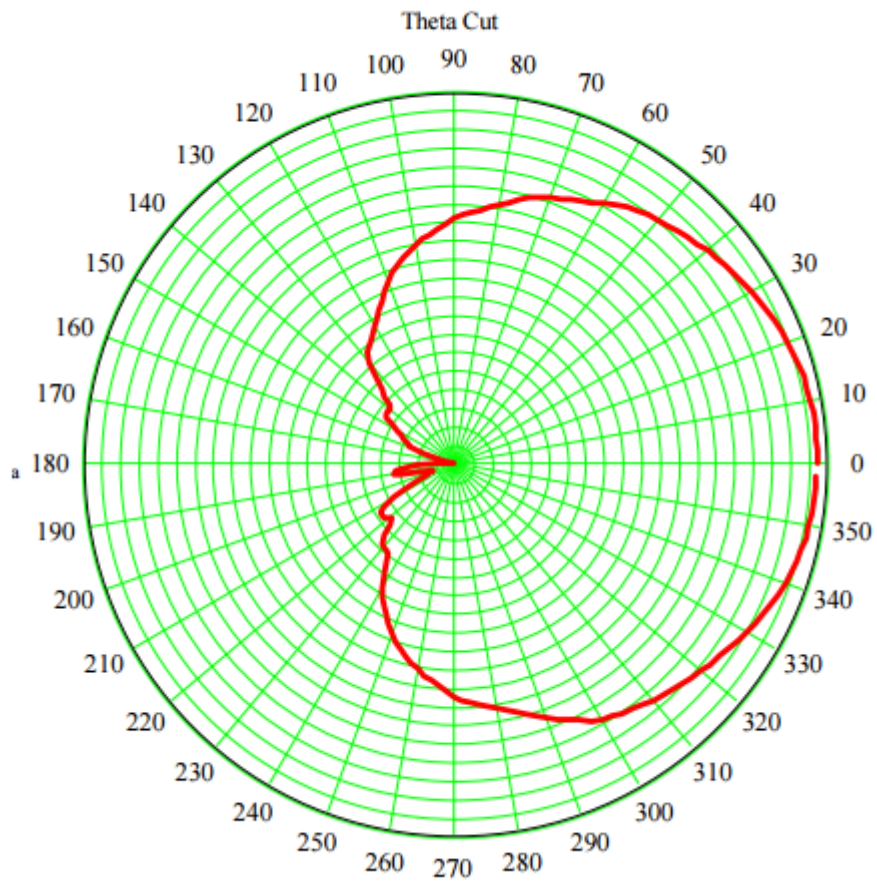
Example XBAND elevation radiation pattern for full size patch ~ 8030 MHz
