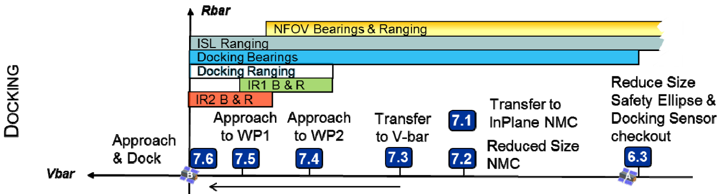
CPOD Vehicle Docking Approach
