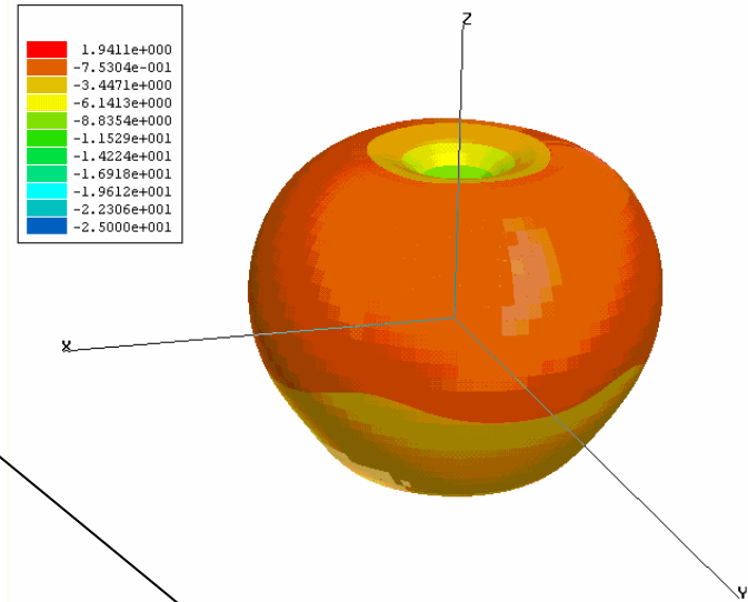
ADPT total (dB) at 2400 MHz. Monopole
