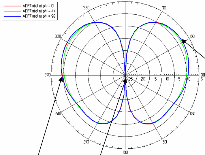
Antenna Directivity Pattern (dB) vs Theta at 2400 MHz, Monopole
