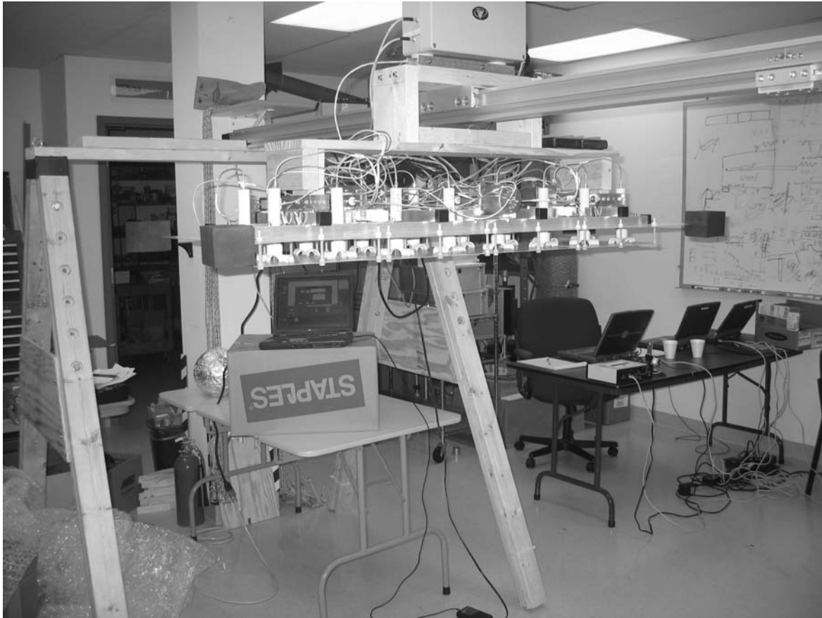
Radar, antenna array, and the supporting structure with 4 m long linear actuator. The array can be moved along the actuator within 2.5 m synthetic aperture. The maximum height of the array above the ground level is 81 in. The minimal height is 48 in.
