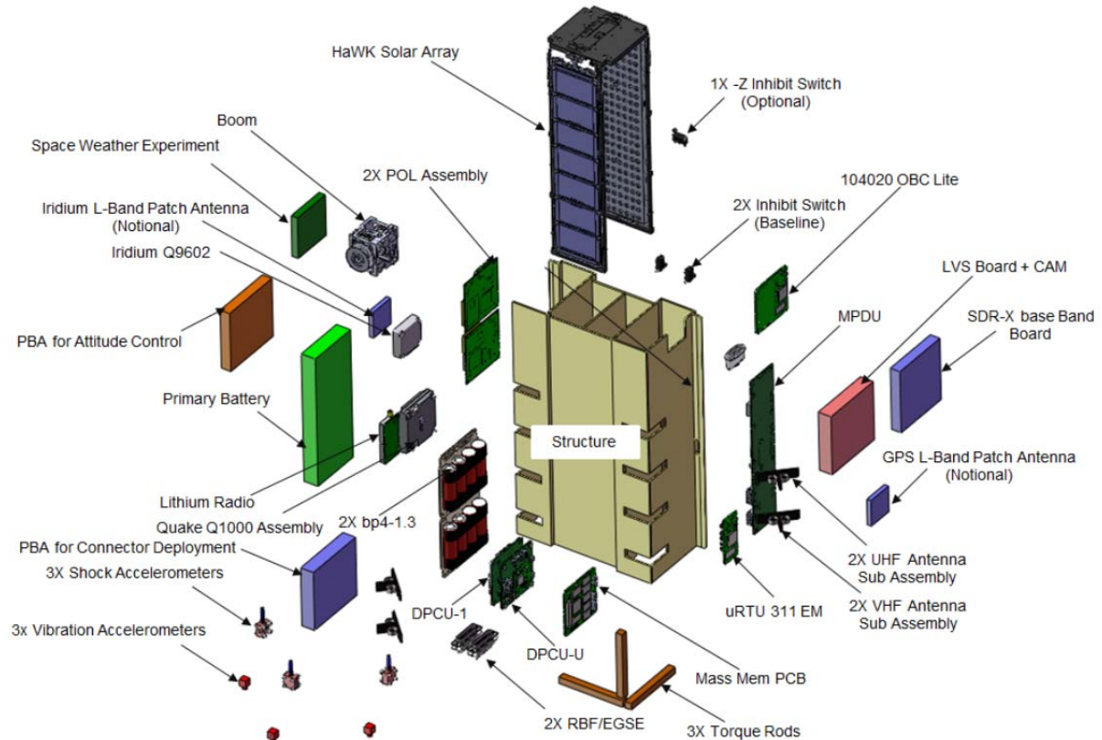
Figure 1: ORS Squared Expanded View
