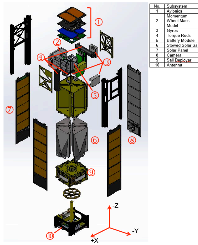
Figure 1: LightSail 2 Expanded View
