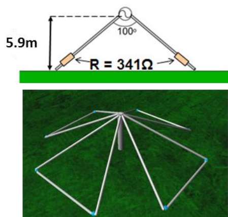
Figure 1. Model Crossed Dipole Antenna (&lt; 20m diameter)
