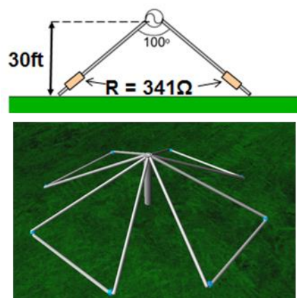
Figure 1a. Model Crossed Dipole Antenna (&lt; 20m diameter)
