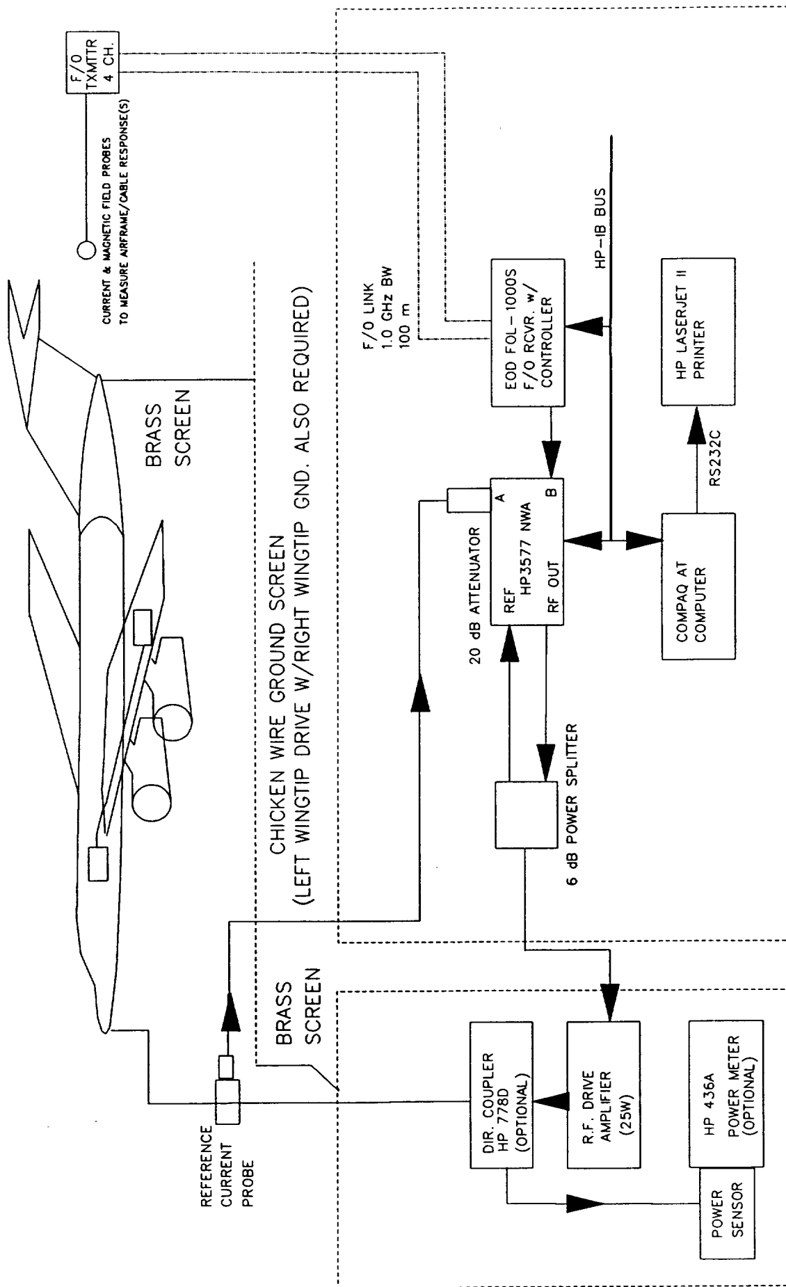
DIRECT DRIVE TEST SETUP (50 Hz - 100 MHz)
