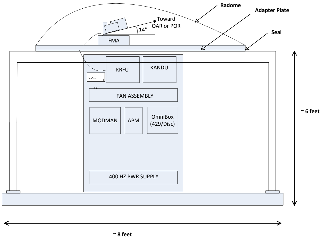
Figure 2: Thales Building 51 RoofTop Ka-Band Antenna System
