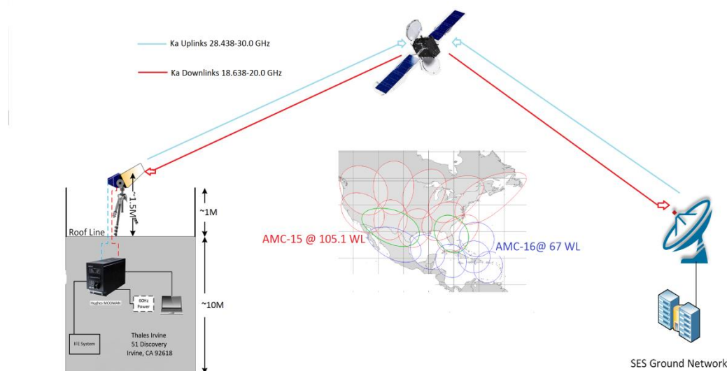
Figure 1: Static MCT Testing on Rooftop of Thales Irvine Building
