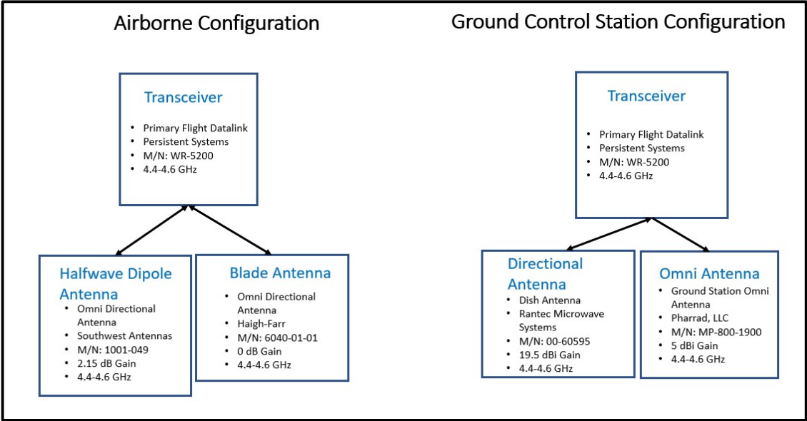
Figure 4: Airborne and Ground Station Configuration
