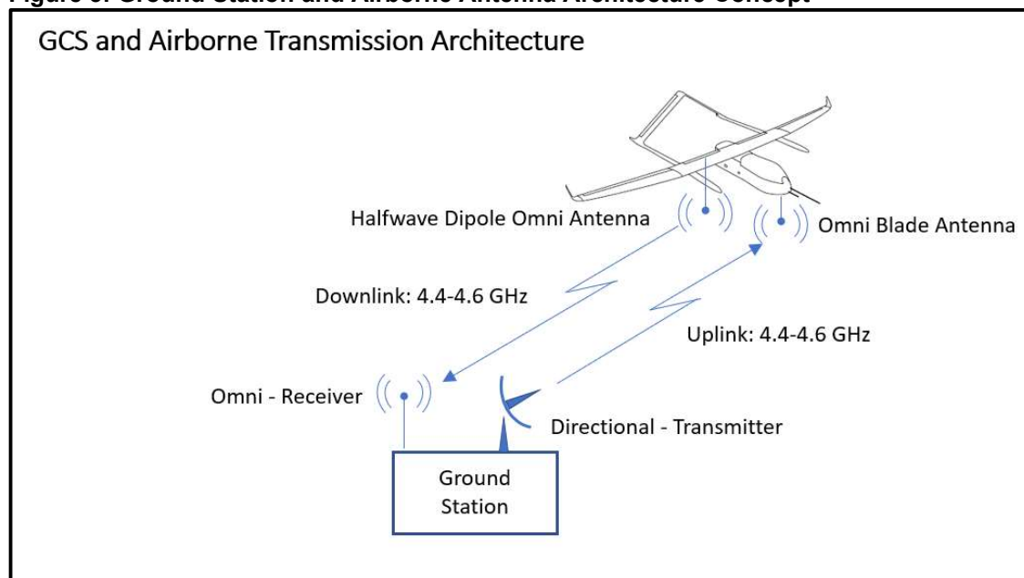
Figure 3: Ground Station and Airborne Antenna Architecture Concept
