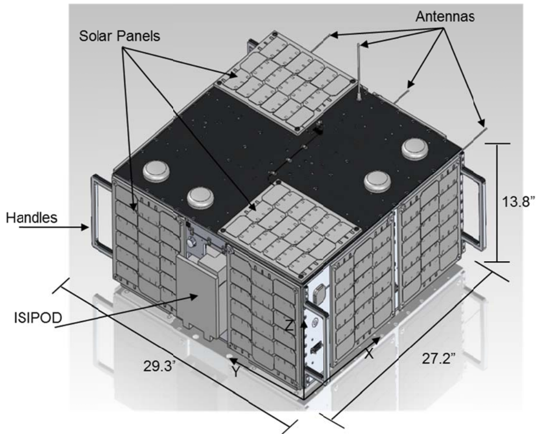
Figure 2-1 AggieSat4 Spacecraft
