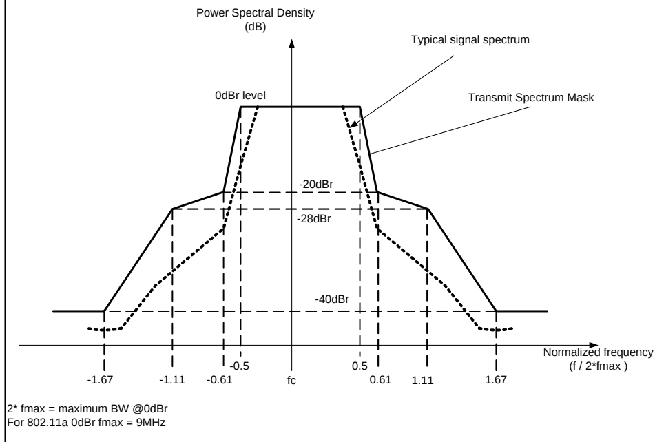
Spectrum Mask (16.5 MHz)
