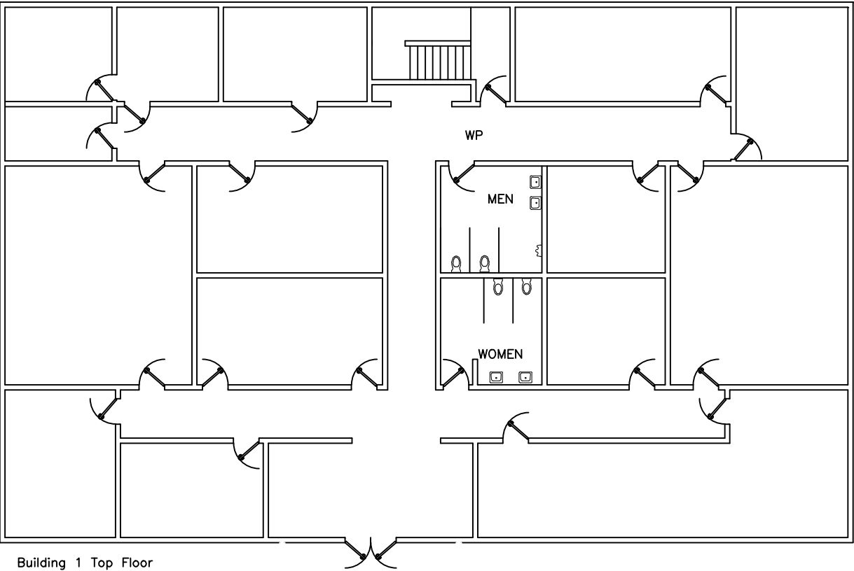
Building 1 Top Floor
