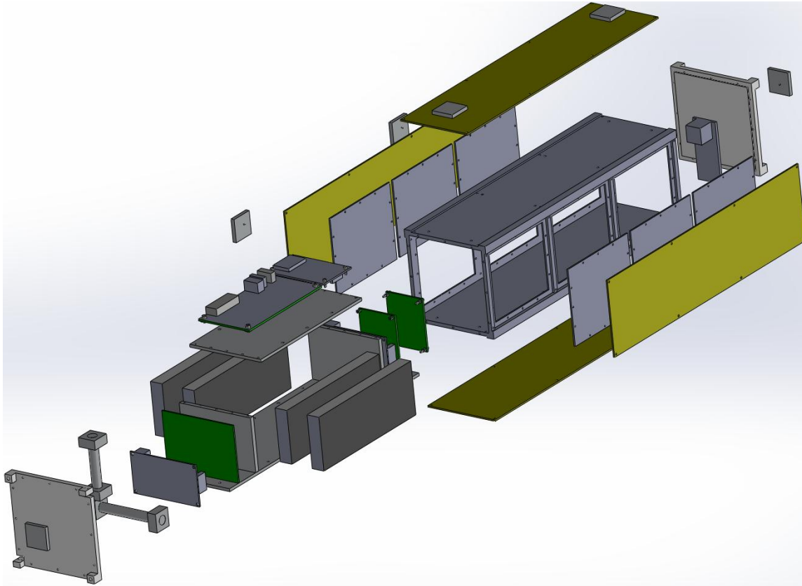
Figure 2: GEARR CubeSat Description
