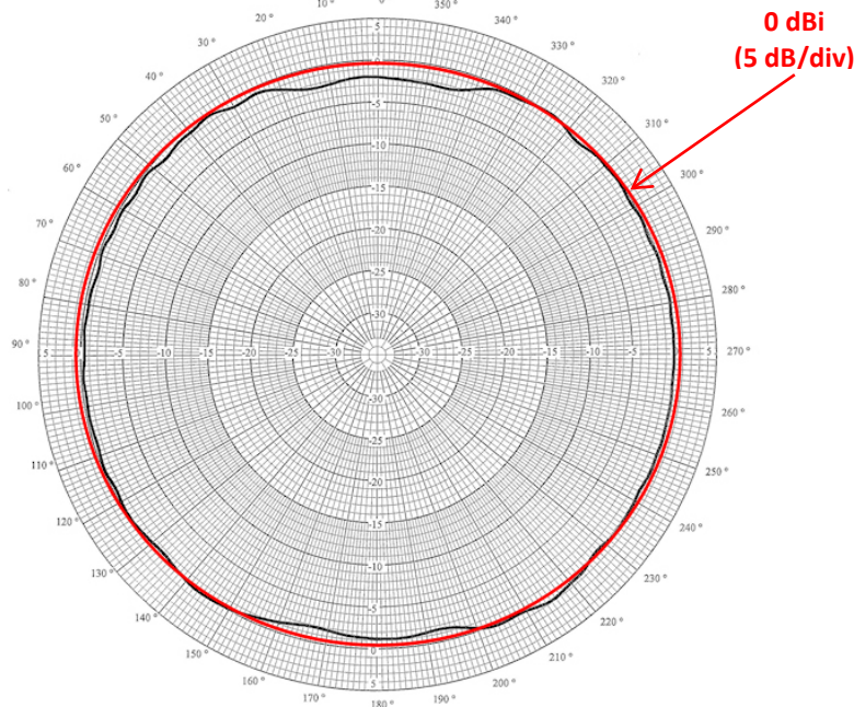
AZIMUTH (YAW) 2.25 GHz
