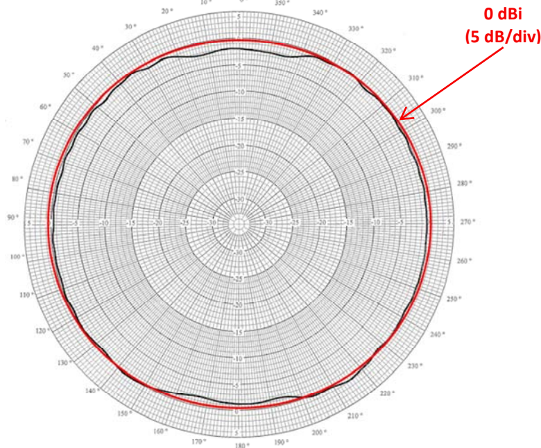
AZIMUTH (YAW) 2.250 GHz
