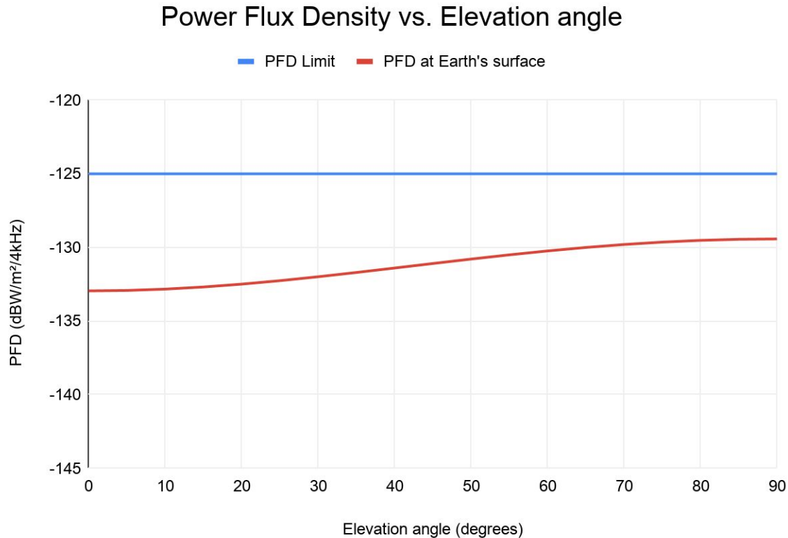
Figure 1. PFD at Earth's surface produced by a satellite transmission. 3
