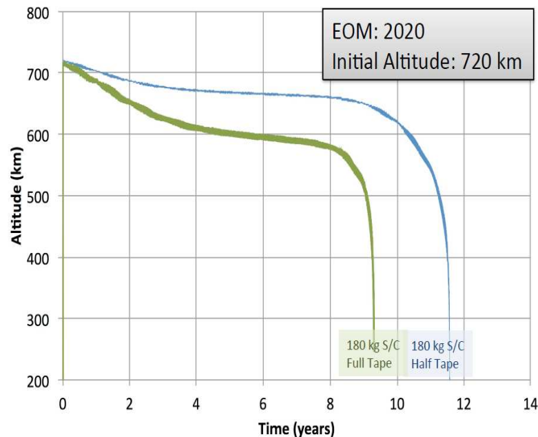
Figure 6-1 OTB re-entry prediction for the full tape length and an illustration of the effect of severing the tape to half length
