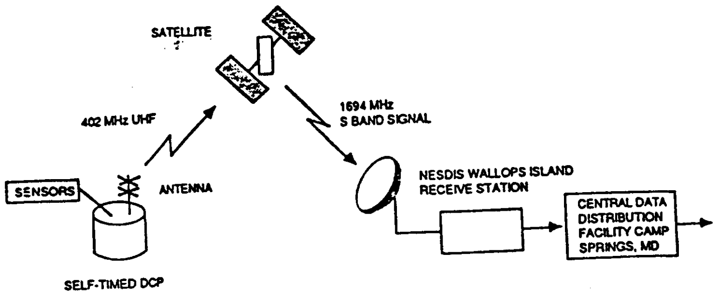
Figure 1.2.1.1 SMS/GOES SELF-TIMED DATA COLLECTION SYSTEM
