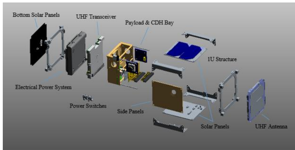
Figure 2 Interior Layout of Argus-02 Components
