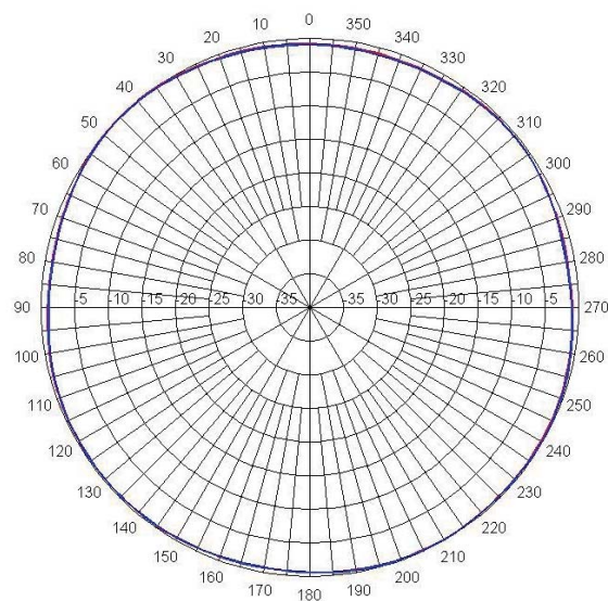
BMUF8043 Azimuth Cut
