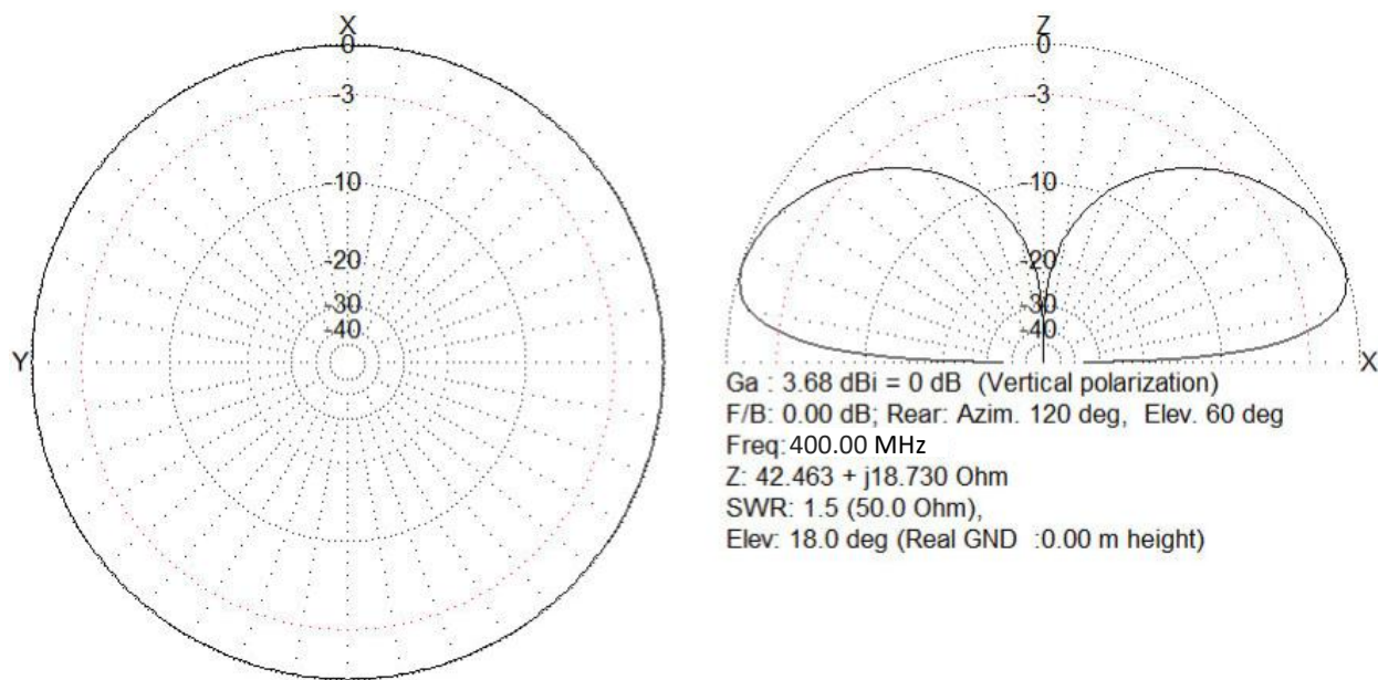
EXTX/EXRX – UHF Experimental Earth Station Antenna Radiation Pattern.
