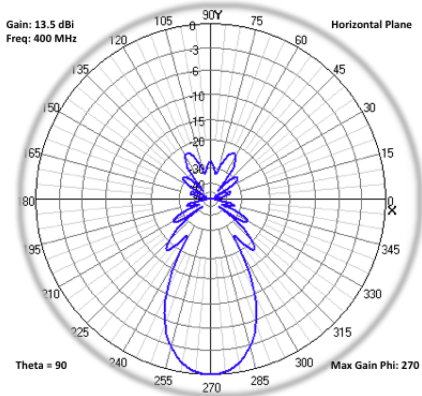
UTX/URX - UHF Earth Station Antenna Radiation Pattern.
