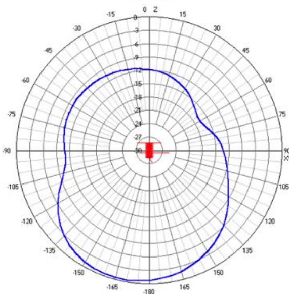
Figure 22 TT&C UHF Satellite Transmit/Receive Antenna Radiation Pattern.
