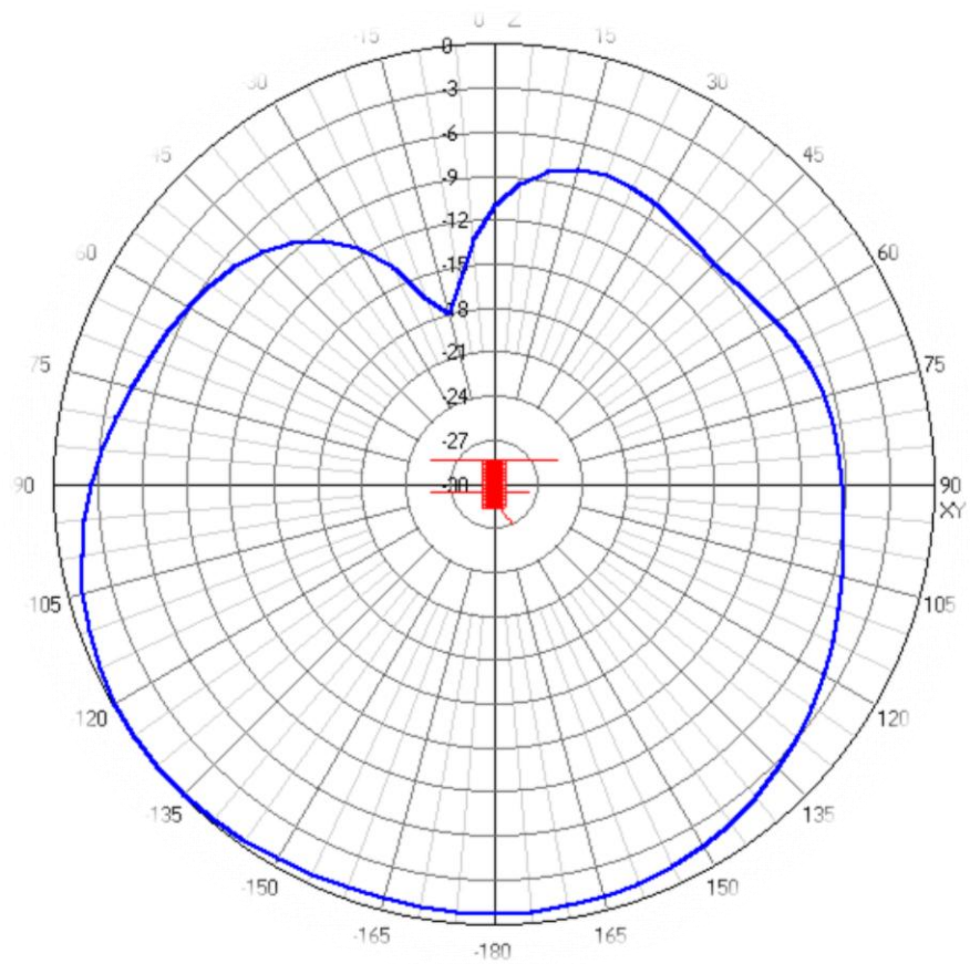
Attachment #1 USATRXX - UHF Satellite Transmit/Receive Radiation Pattern.
