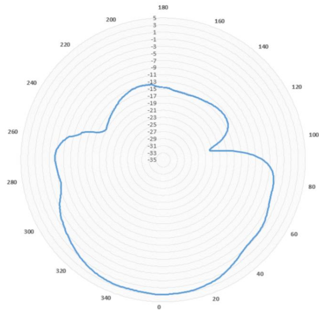
Figure 20 Flexitech Broadband Receive Antenna and Radiation Pattern.
