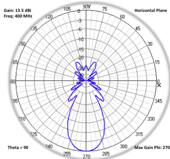
Figure 23 UHF Earth Station Antenna Radiation Pattern.
