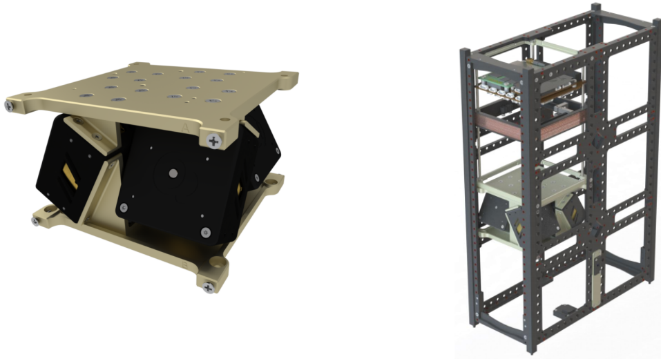
Figure 4. Reaction wheel system and its internal place on SAI-2.
