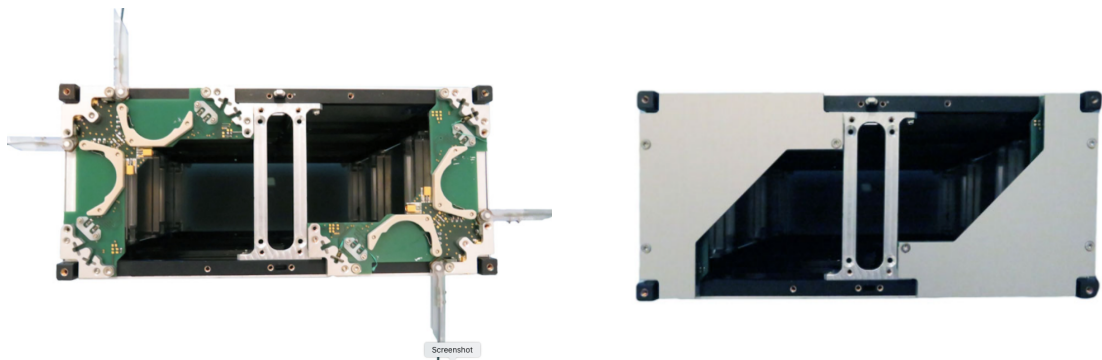
Figure 3. SAI-2 TT&C Commns Antenna Details
