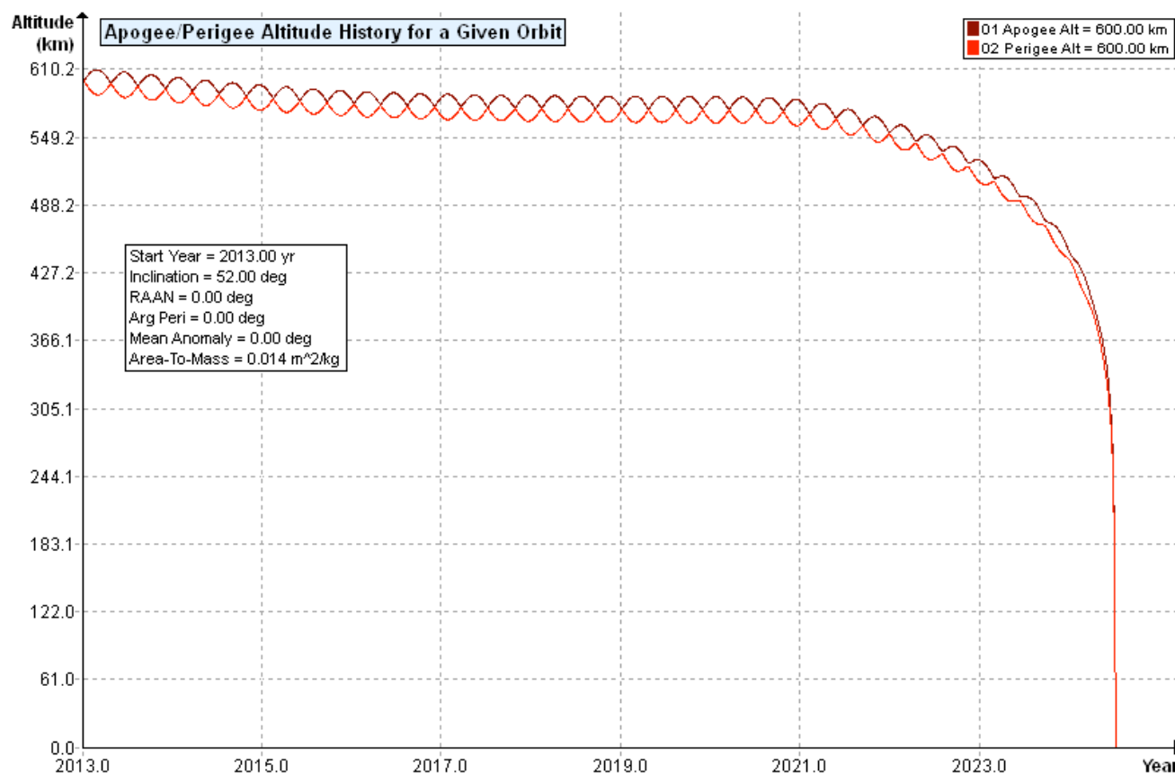
Figure 3. SkyCube orbit history, assuming no balloon inflation after orbit insertion at T=2013.0 .
