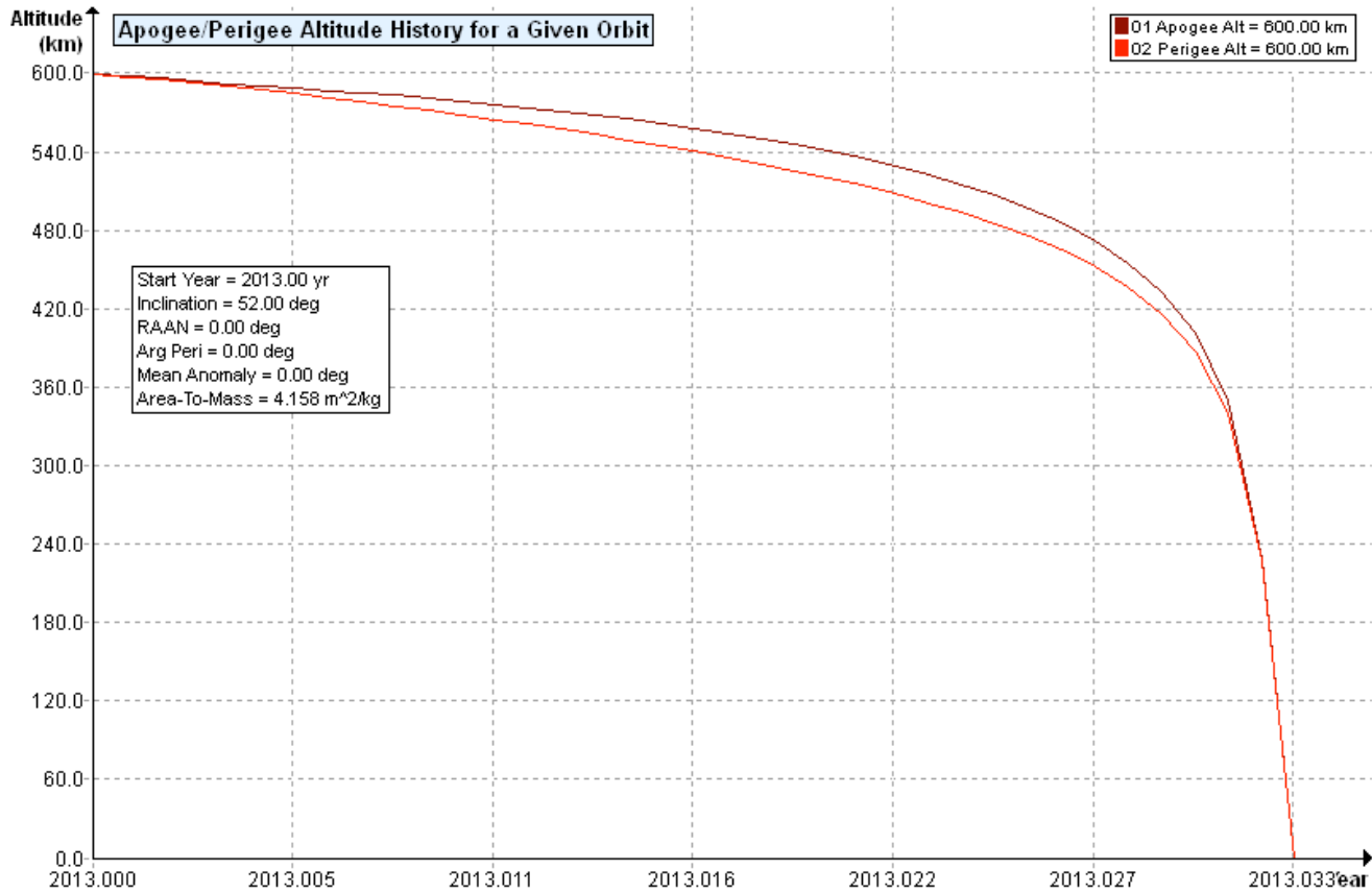
Figure 2. SkyCube orbit history, assuming successful balloon inflation immediately upon orbit insertion at T=2013.0
