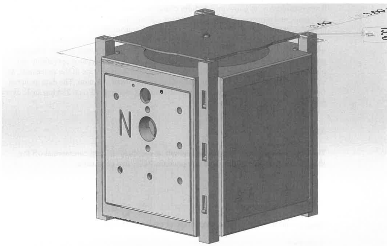
Figure 2: EdgeCube assembled view (w/o antenna)
