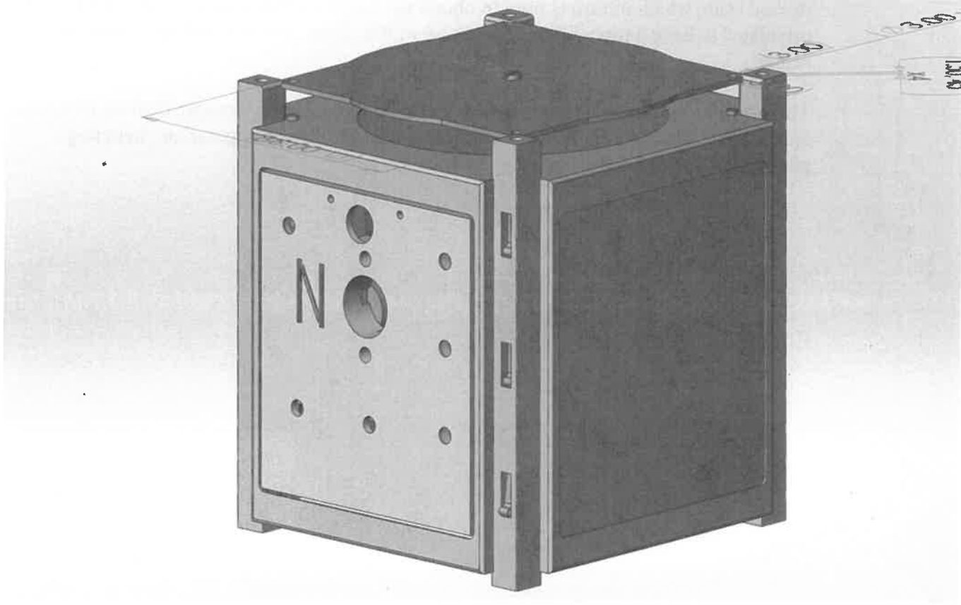
Figure 4: EdgeCube Assembled View (w/o antenna)
