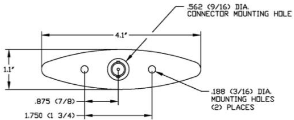
MOUNTING INFORMATION
