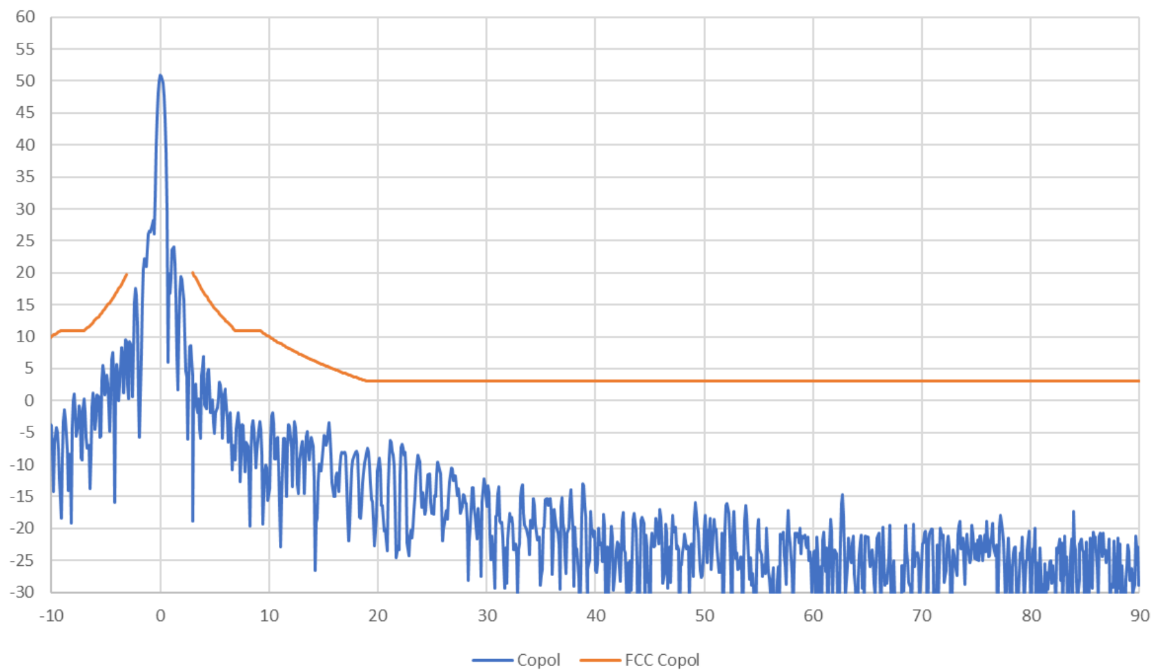
AvL 2.2m Ka Band Antenna 19.3 GHz RHCP Elevation Pattern
