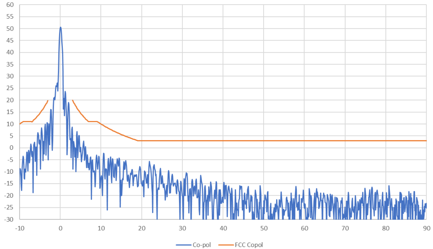
AvL 2.2m Ka Band Antenna 18.568 GHz RHCP Elevation Pattern
