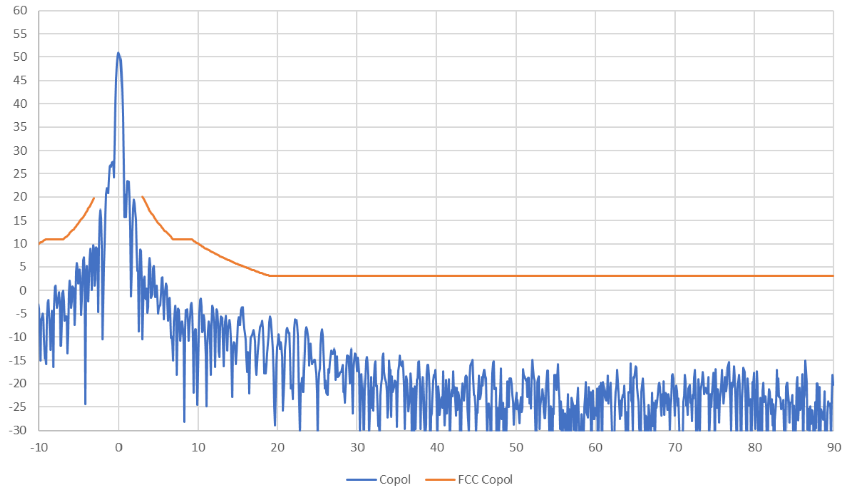
AvL 2.2m Ka Band Antenna 19.3 GHz LHCP Elevation Pattern
