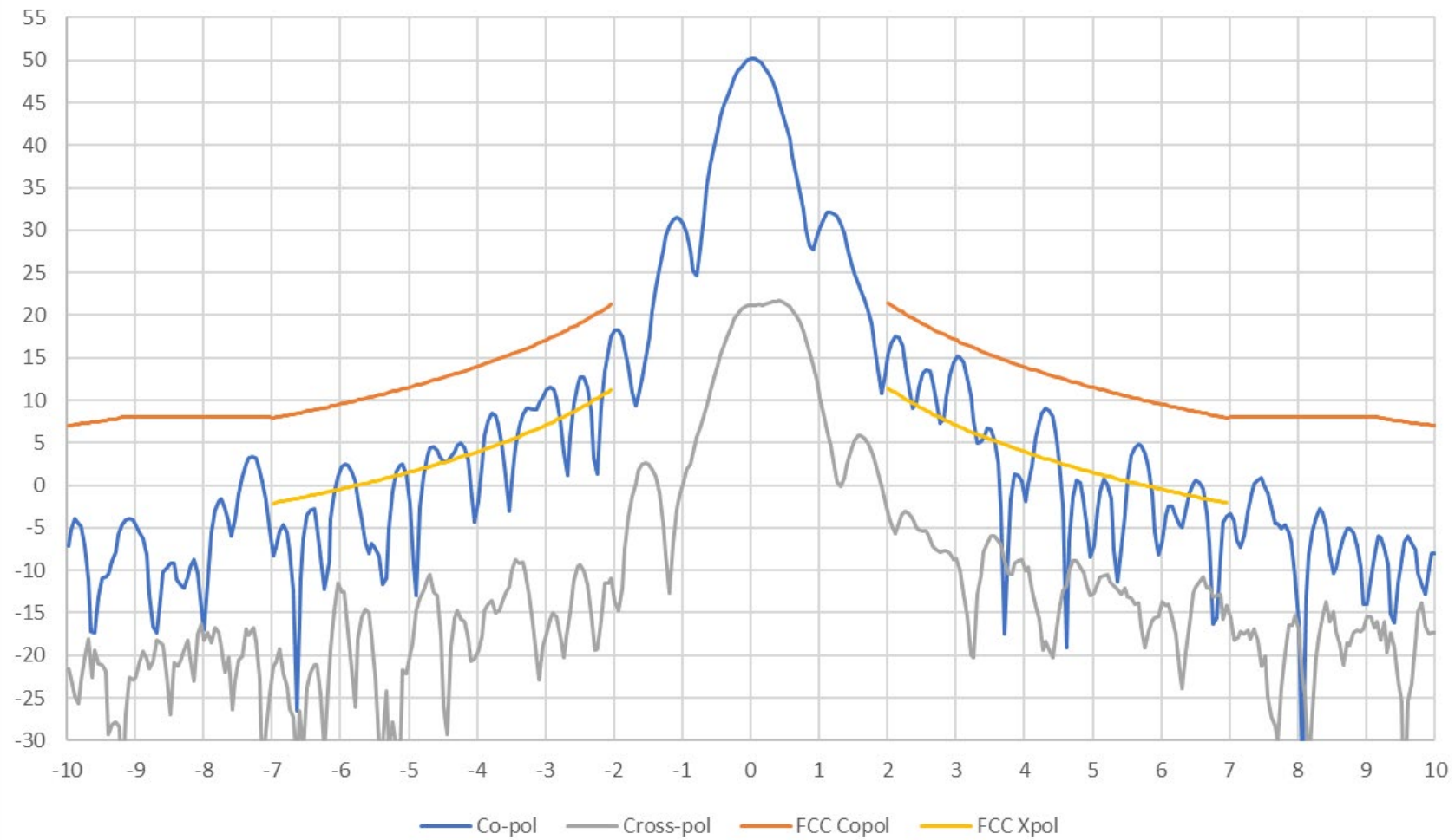
AvL 2.2m Ka Band Antenna 17.835 GHz LHCP Azimuth Pattern
