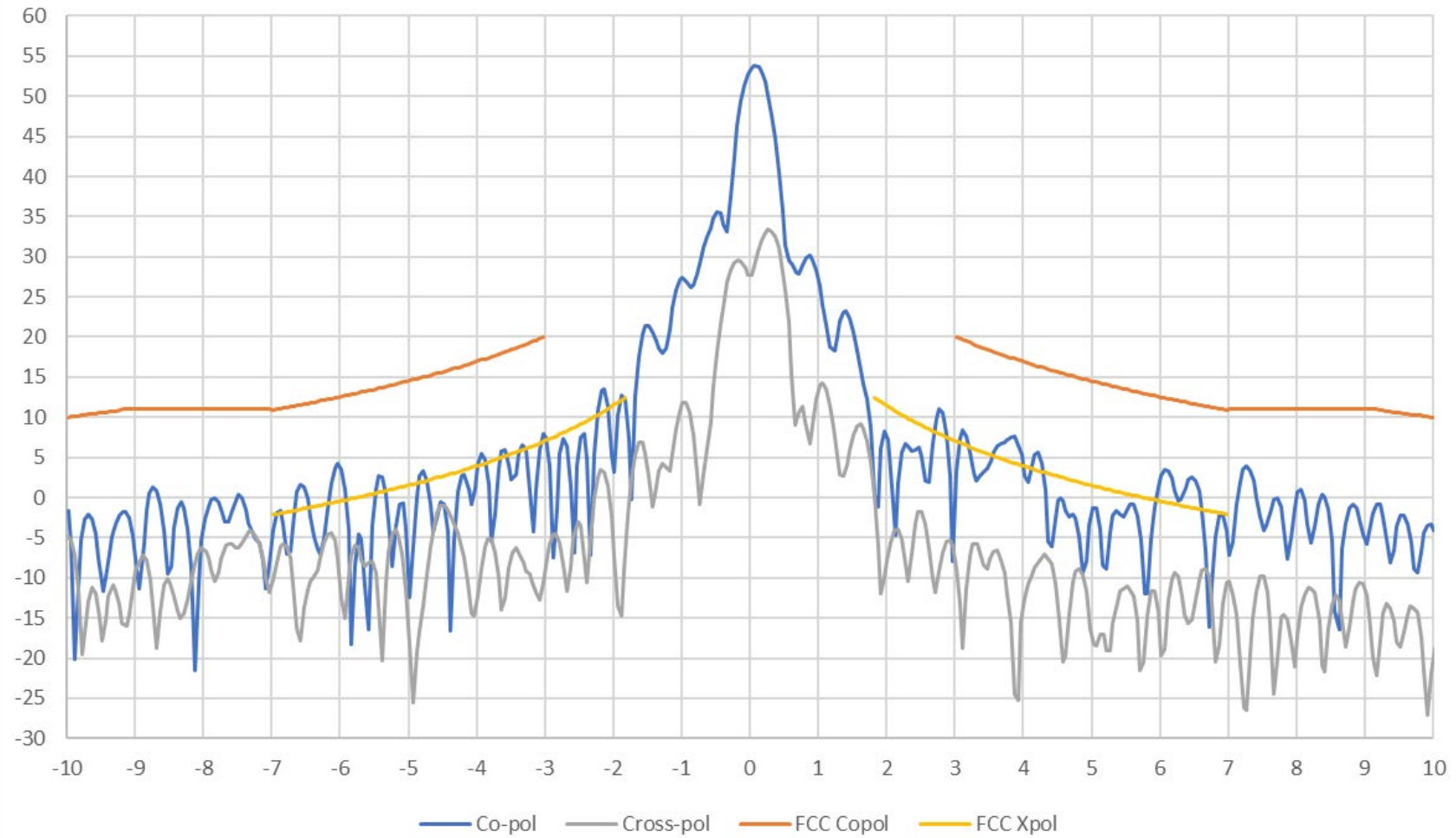
AvL 2.2m Ka Band Antenna 27.635 GHz LHCP Elevation Pattern
