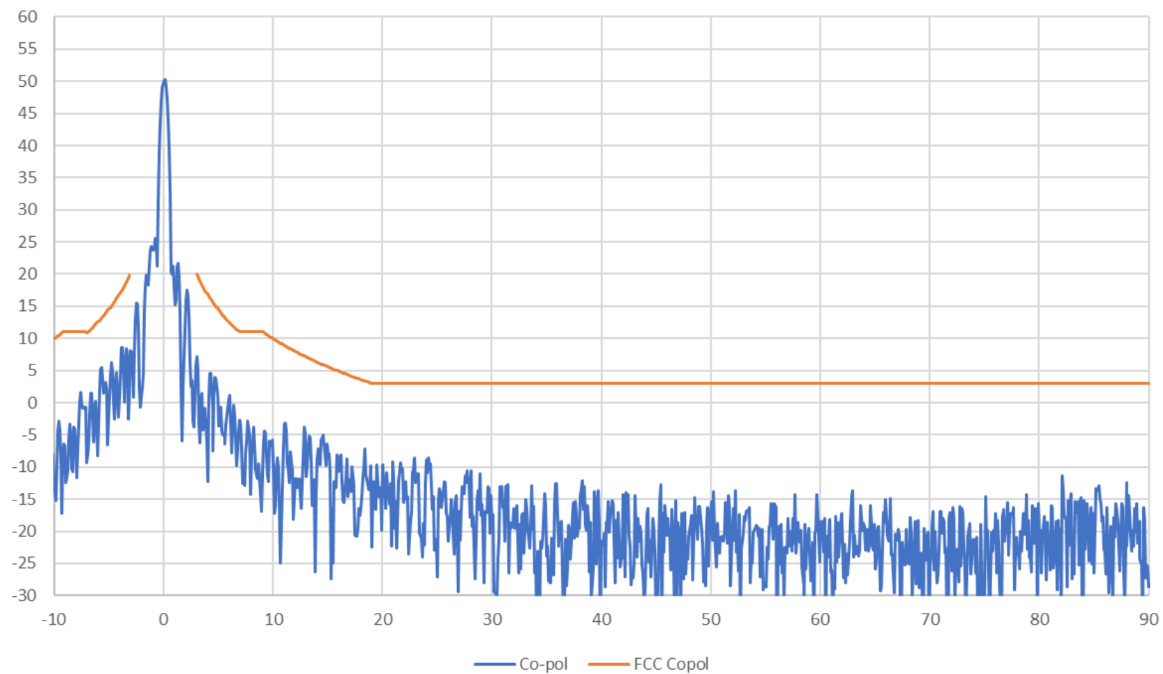
AvL 2.2m Ka Band Antenna 17.835 GHz RHCP Elevation Pattern
