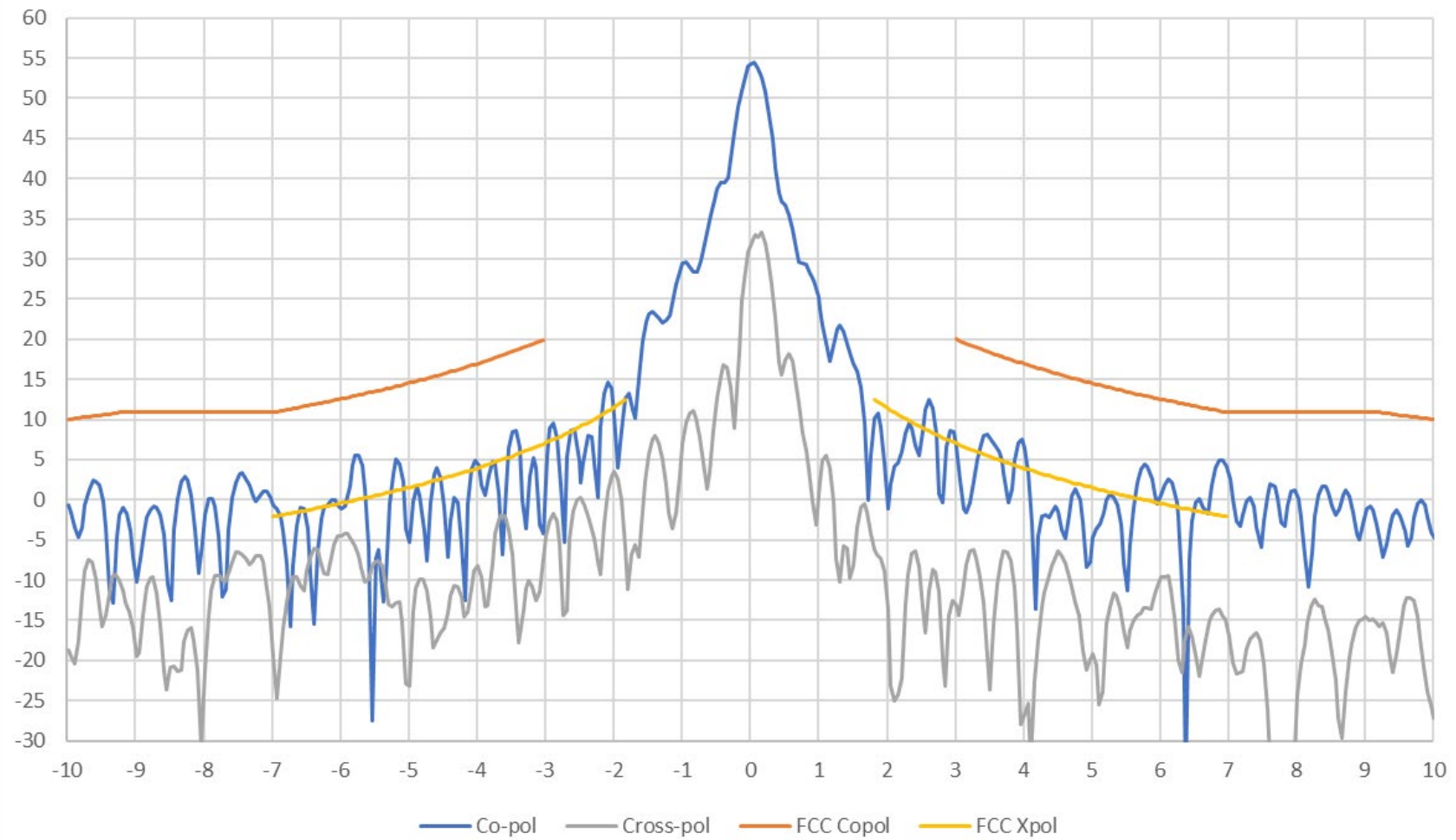
AvL 2.2m Ka Band Antenna 29.09 GHz RHCP Elevation Pattern
