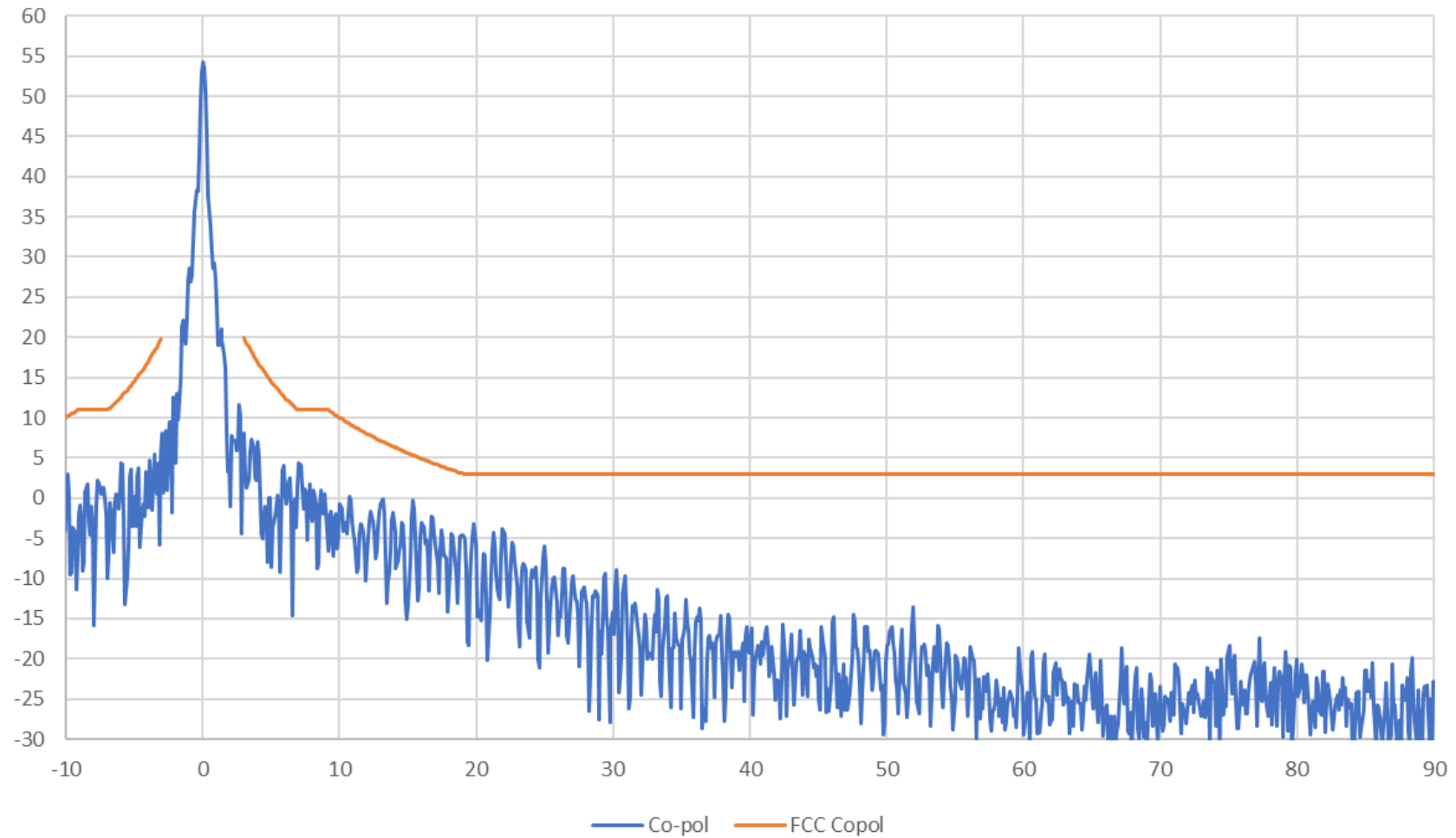
AvL 2.2m Ka Band Antenna 28.363 GHz RHCP Elevation Pattern
