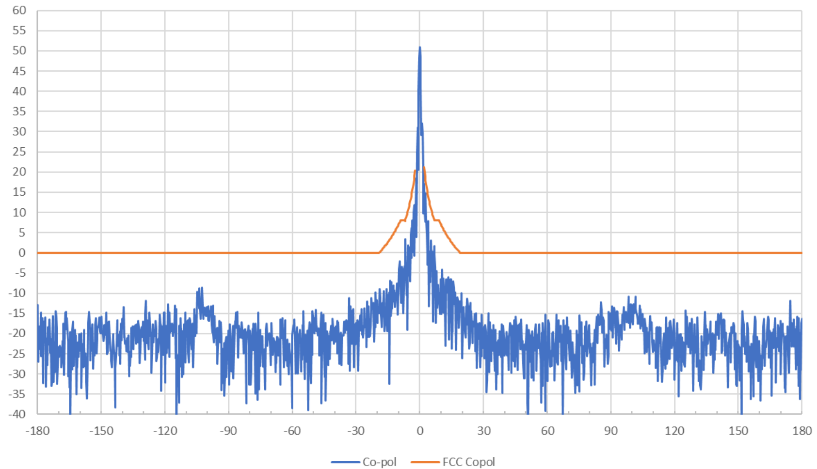
AvL 2.2m Ka Band Antenna 19.3 GHz LHCP Azimuth Pattern
