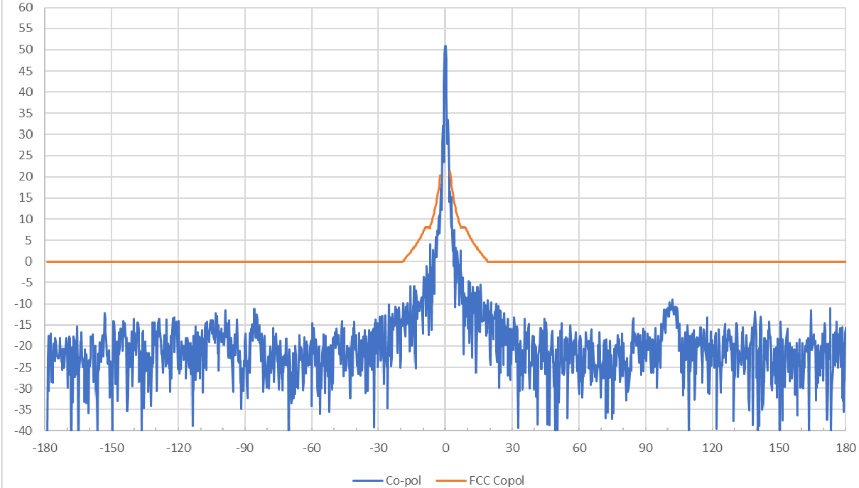
AvL 2.2m Ka Band Antenna 19.3 GHz RHCP Azimuth Pattern
