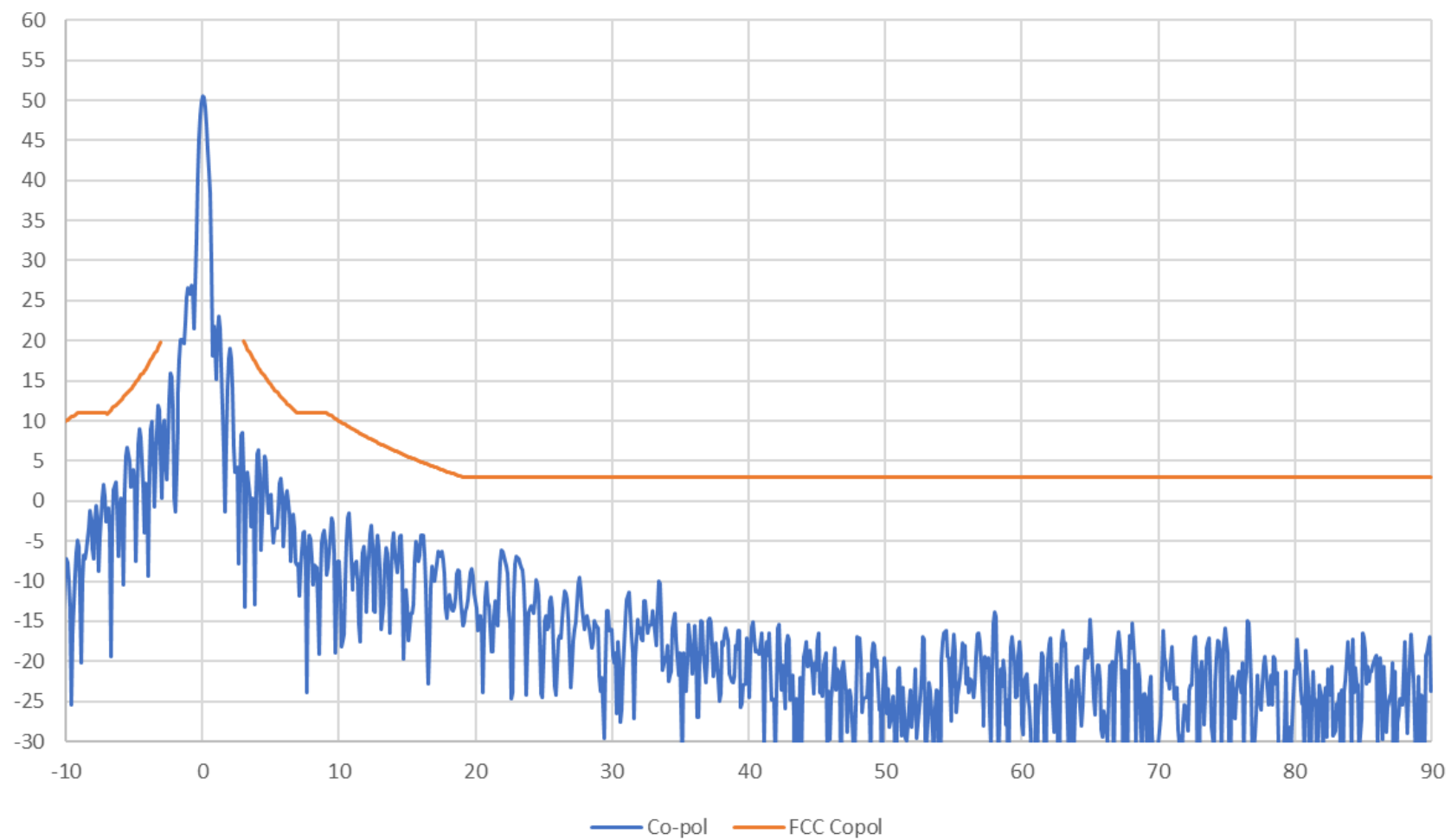
AvL 2.2m Ka Band Antenna 18.568 GHz LHCP Elevation Pattern
