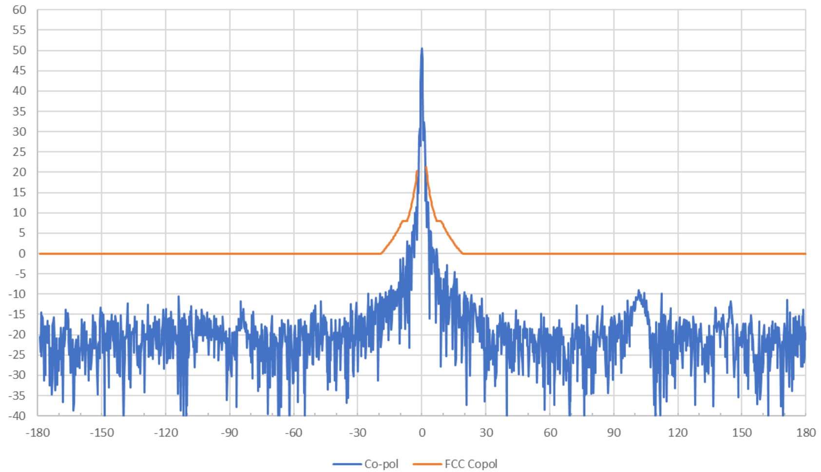
AvL 2.2m Ka Band Antenna 18.568 GHz RHCP Azimuth Pattern
