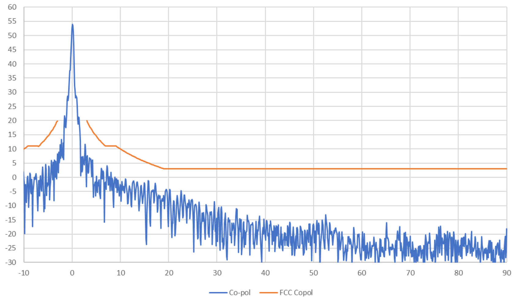
AvL 2.2m Ka Band Antenna 27.635 GHz RHCP Elevation Pattern
