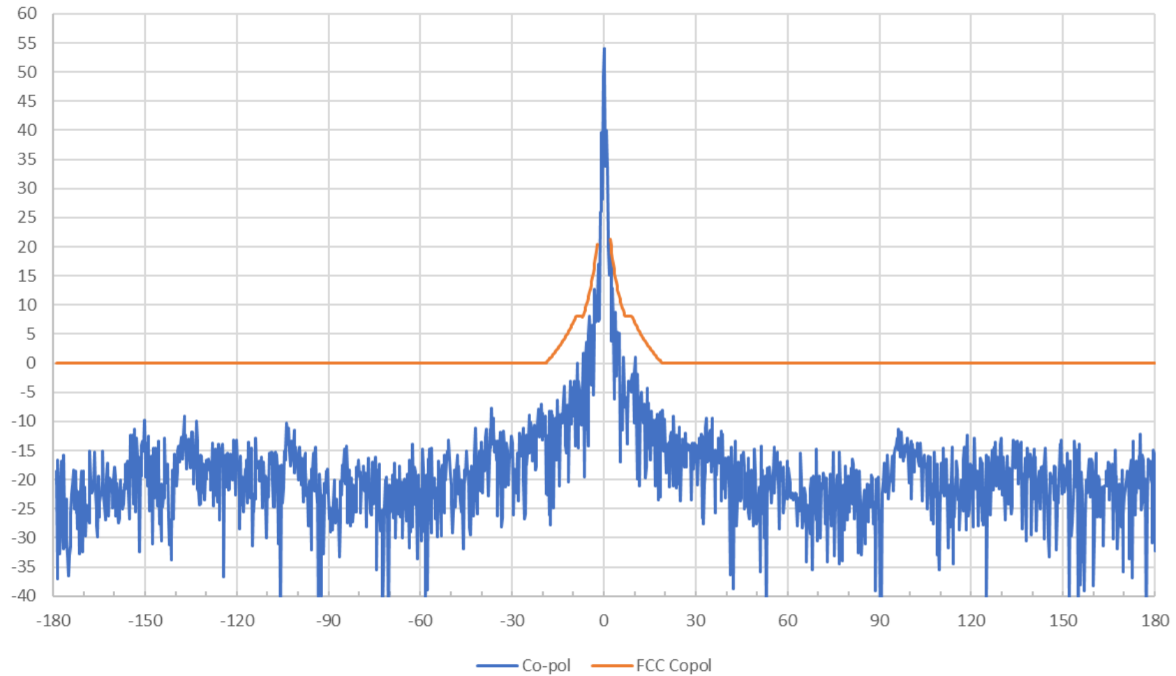
AvL 2.2m Ka Band Antenna 27.635 GHz LHCP Azimuth Pattern
