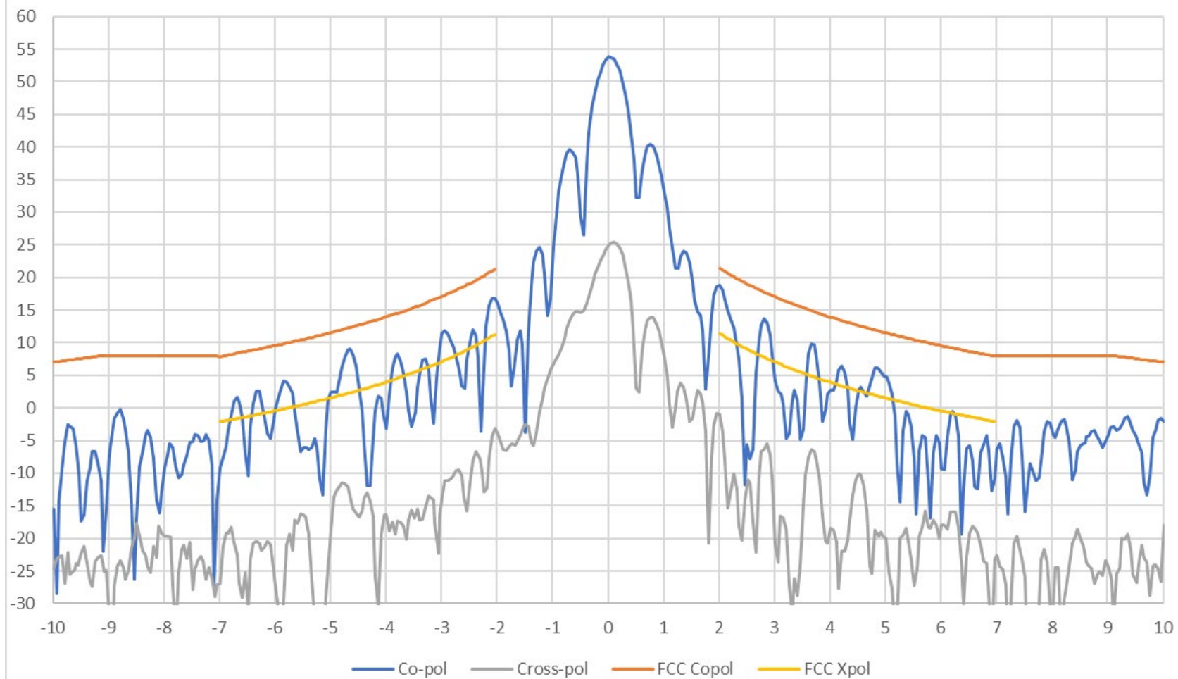
AvL 2.2m Ka Band Antenna 27.635 GHz RHCP Azimuth Pattern
