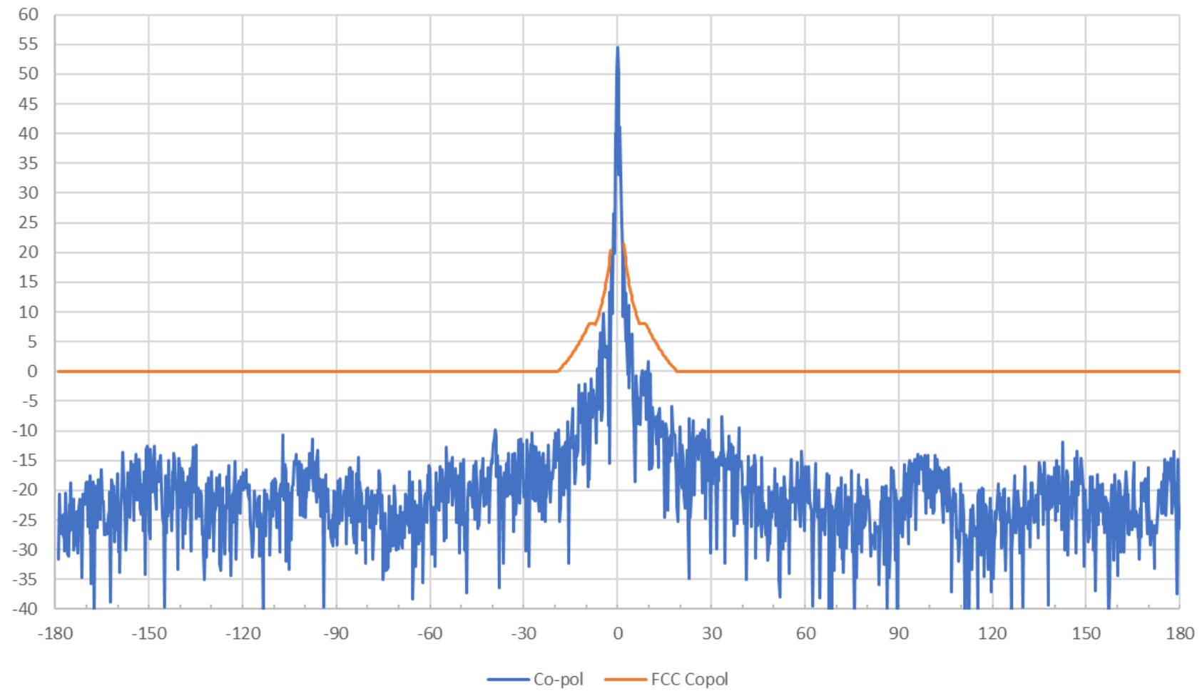
AvL 2.2m Ka Band Antenna 29.09 GHz LHCP Azimuth Pattern
