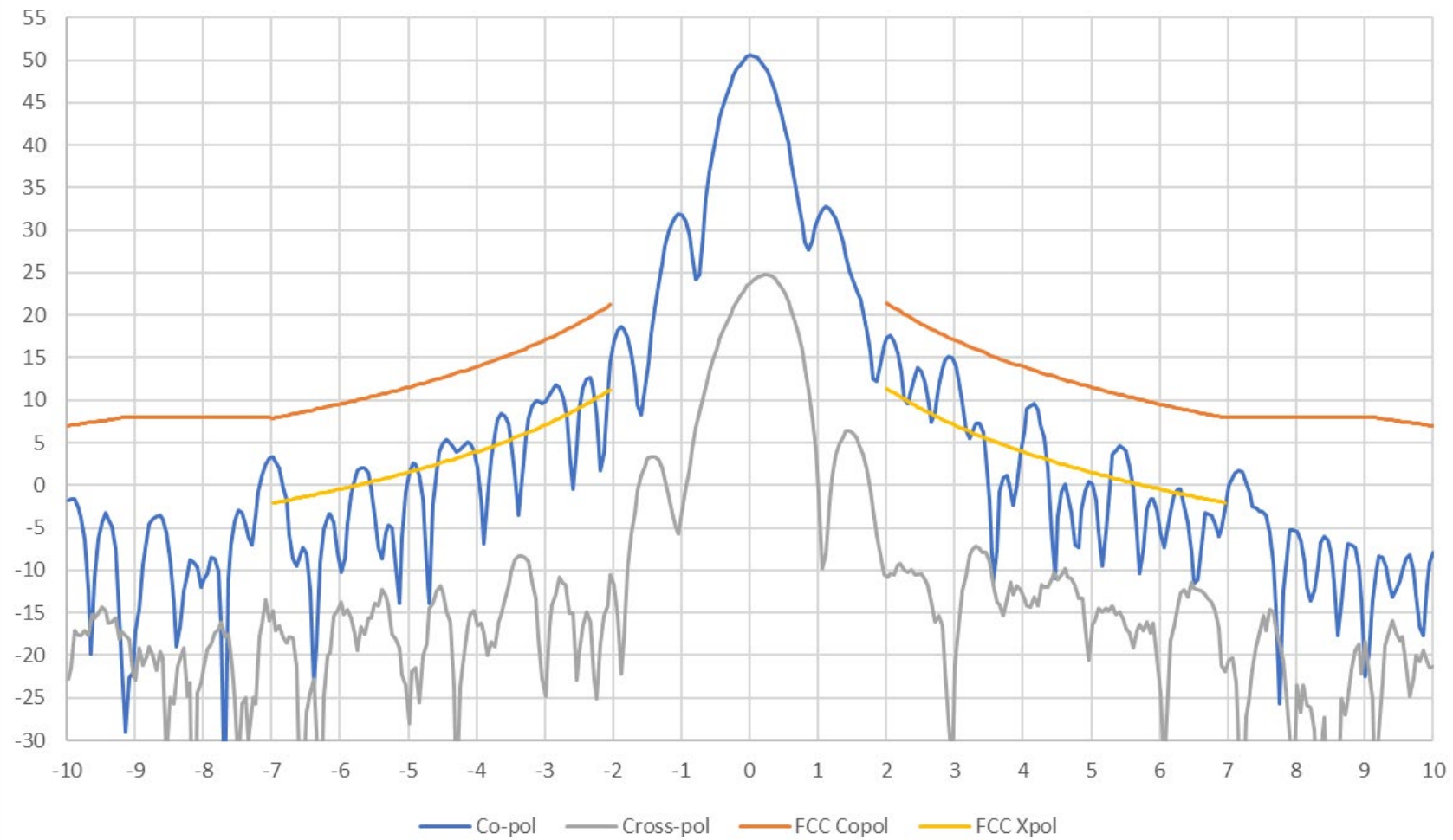
AvL 2.2m Ka Band Antenna 18.568 GHz LHCP Azimuth Pattern
