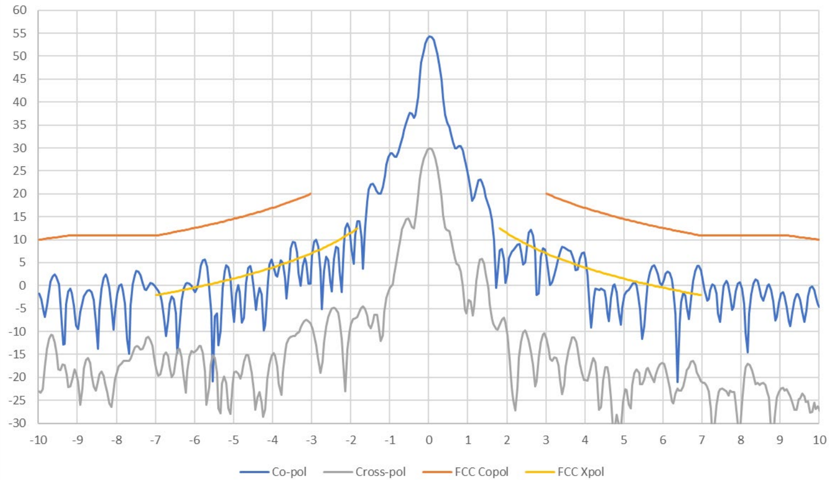
AvL 2.2m Ka Band Antenna 29.09 GHz LHCP Elevation Pattern
