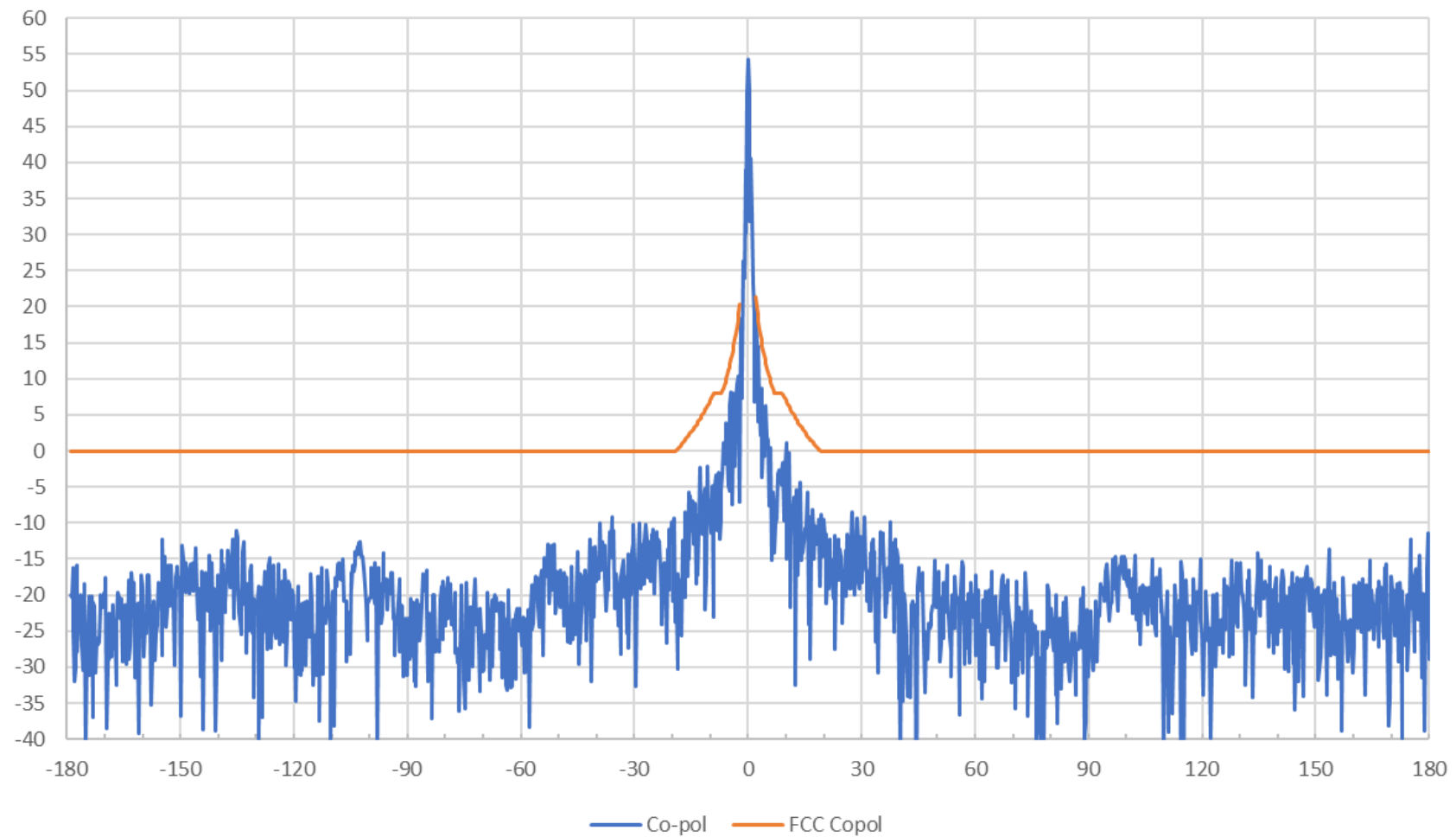
AvL 2.2m Ka Band Antenna 28.363 GHz LHCP Azimuth Pattern
