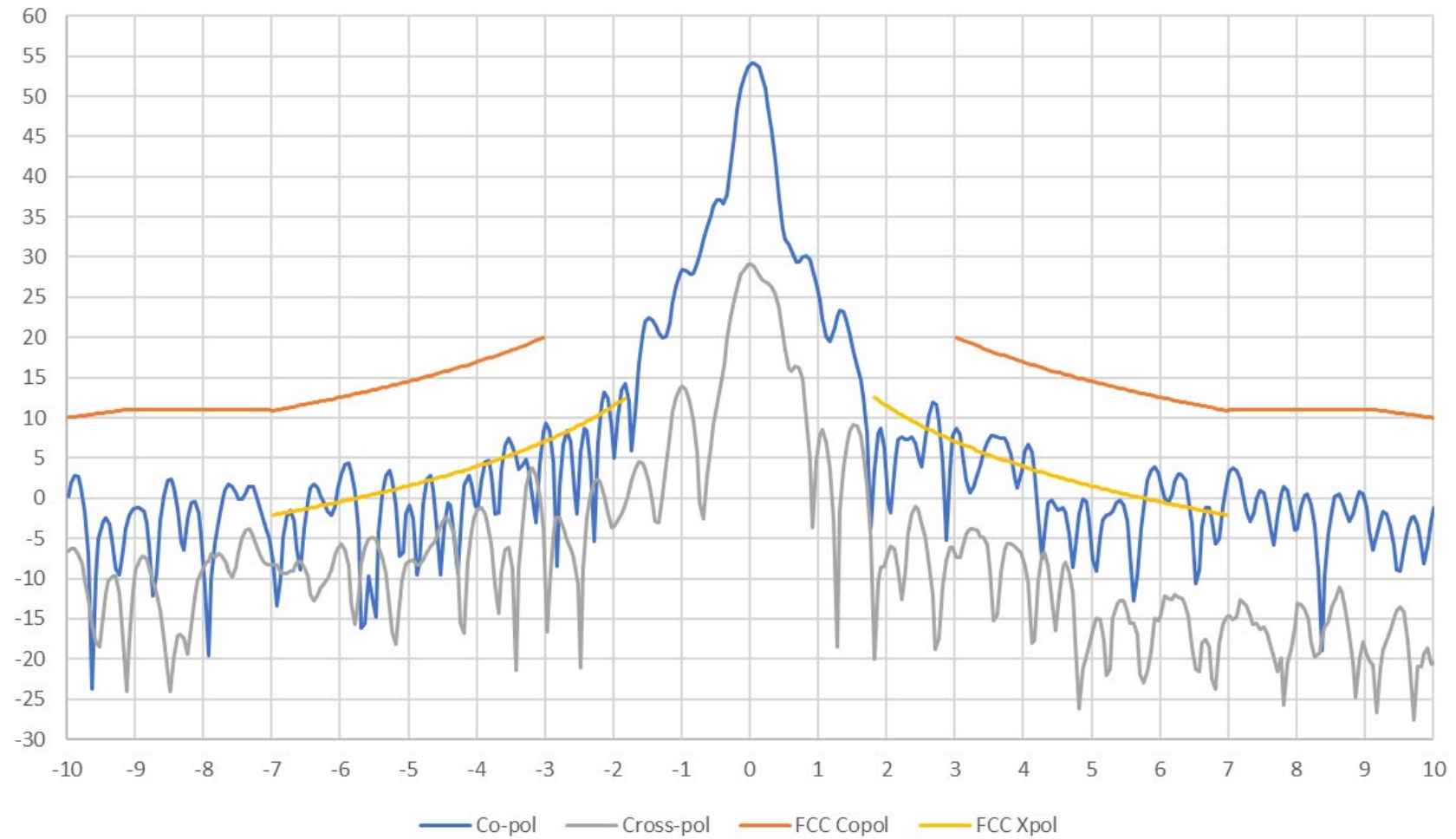
AvL 2.2m Ka Band Antenna 28.363 GHz LHCP Elevation Pattern
