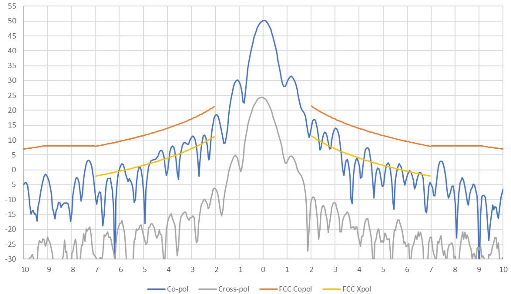
AvL 2.2m Ka Band Antenna 17.835 GHz RHCP Azimuth Pattern
