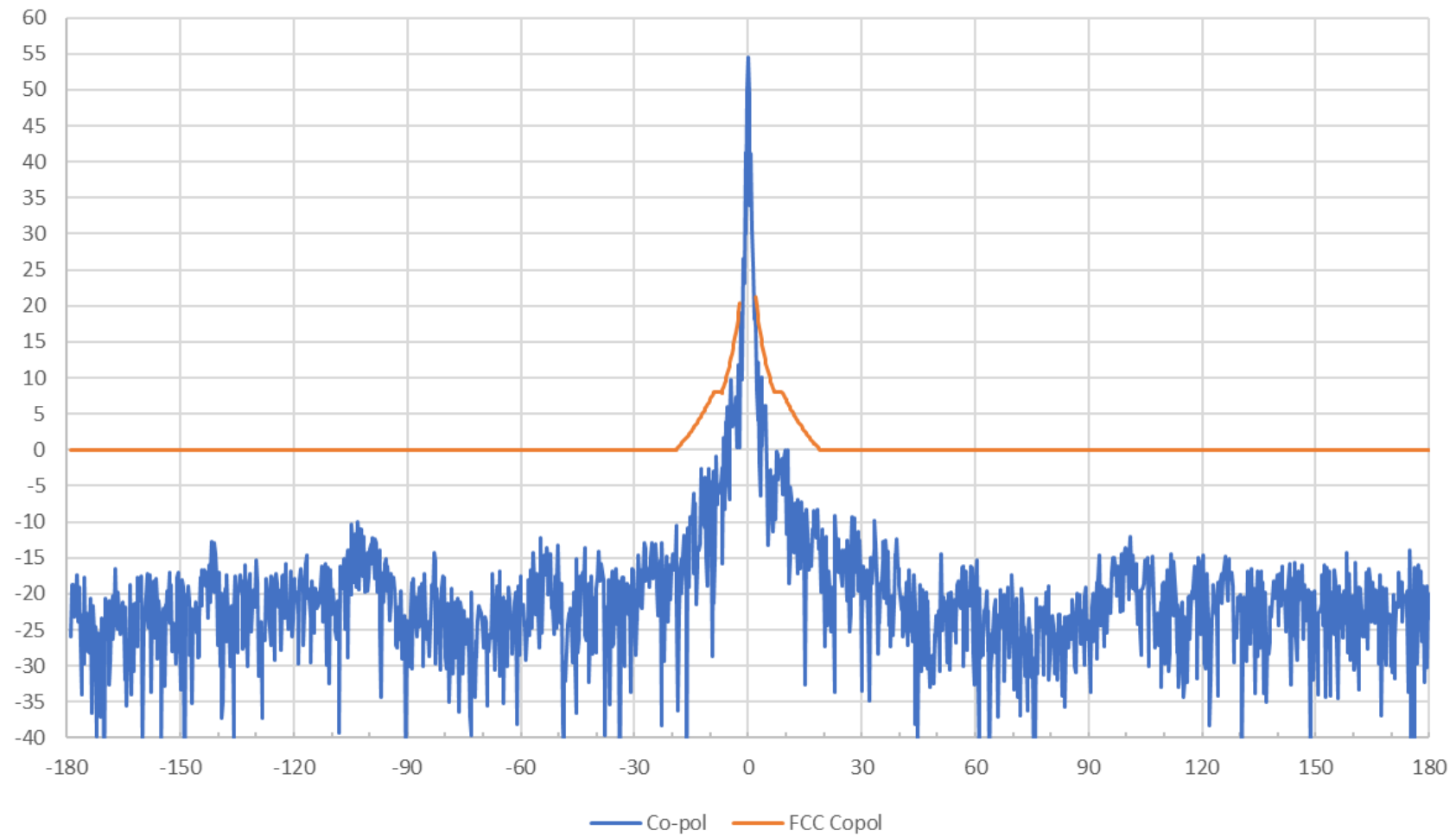
AvL 2.2m Ka Band Antenna 29.09 GHz RHCP Azimuth Pattern
