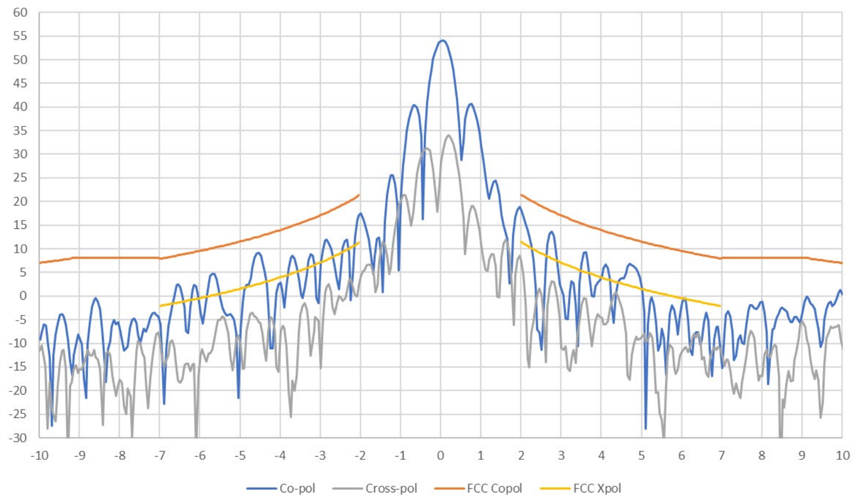
AvL 2.2m Ka Band Antenna 28.363 GHz RHCP Azimuth Pattern
