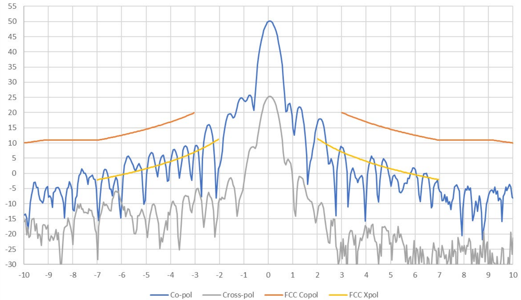
AvL 2.2m Ka Band Antenna 17.835 GHz LHCP Elevation Pattern
