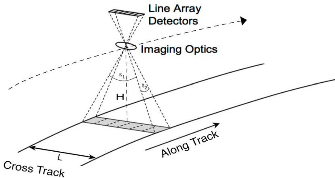
Figure 5: Push broom imaging geometry.
