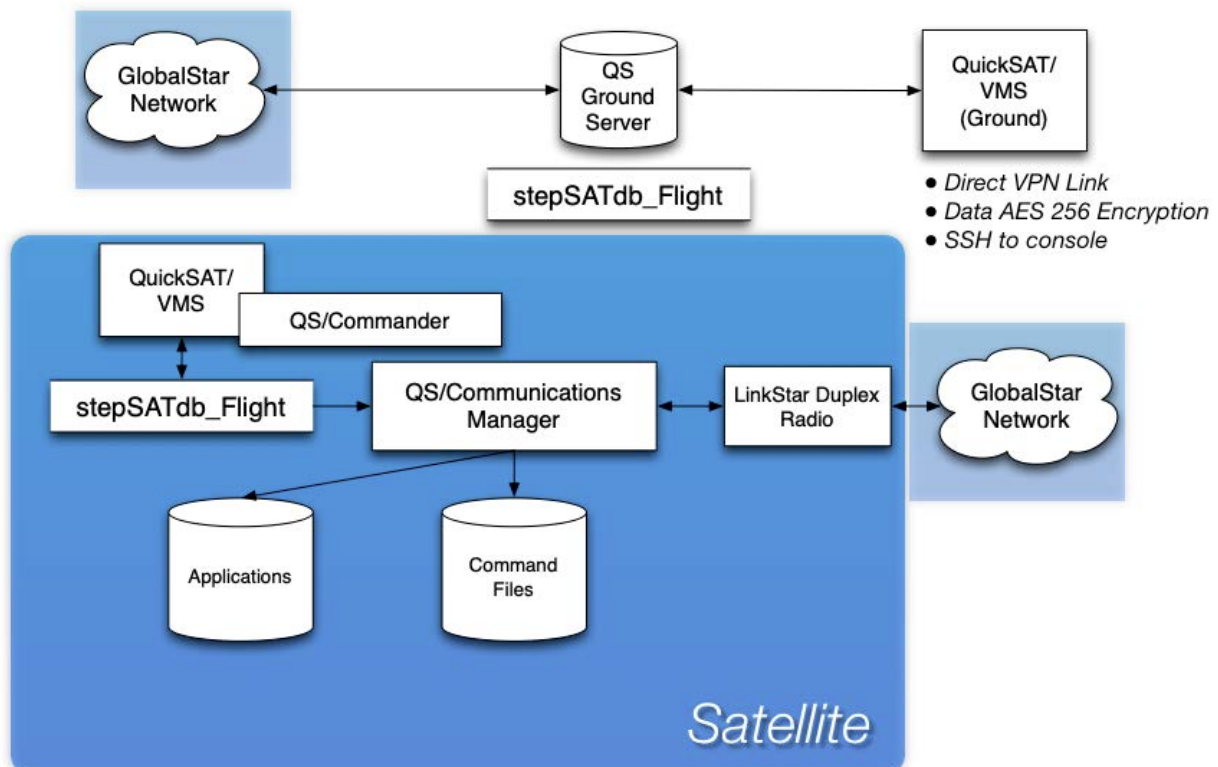
Figure 10: Ground to Satellite/Satellite to Ground Communications via QuickSAT through the GSP-1720 summary view
