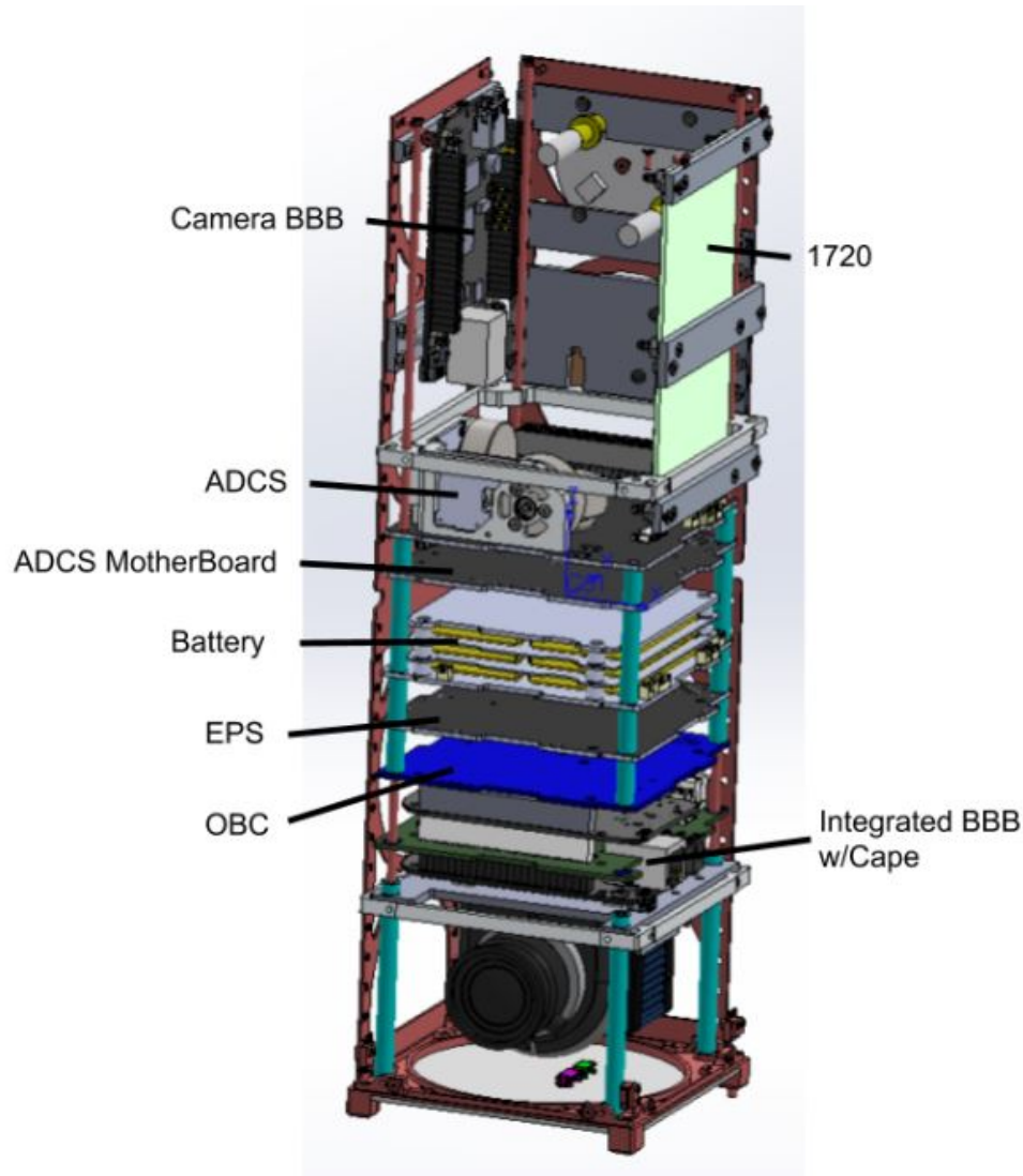
Figure 9: The CaNOP satellite and supporting systems.
