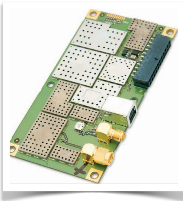
Figure 7: The LinkStar GSP-1720 duplex radio providing internet based communications.
