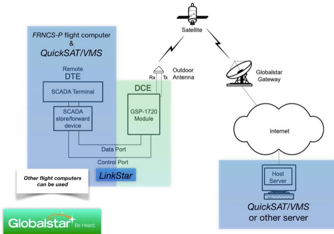
Figure 10: Baseline Communications Scheme with LinkStar duplex radio
