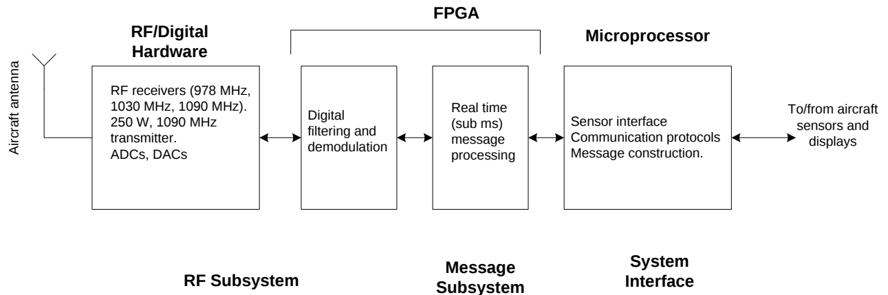
Transponder LRU Block Diagram
