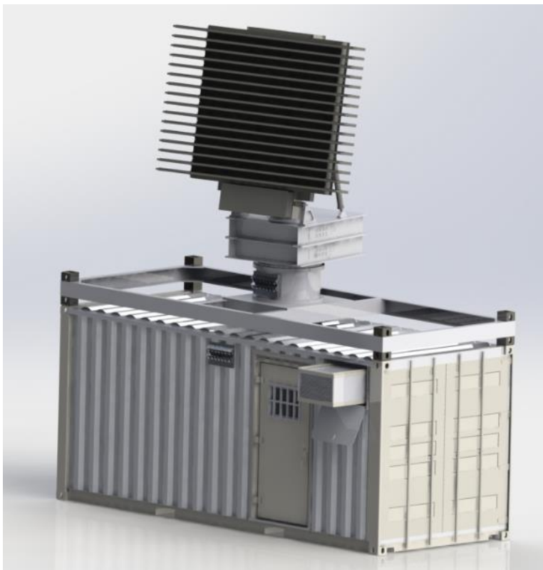
Weber Array mounted above 20 foot ISO shipping container
