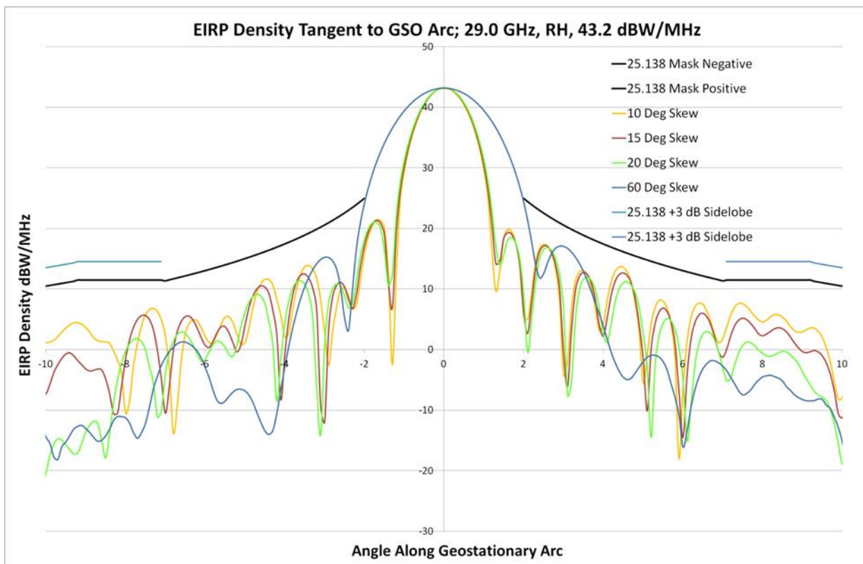
Figure 11 – EIRP Density tangent to GSO Arc, 29.0 GHz, RHP, 43.2 dBW/MHz, -10 to +10 deg., 25.138(a)(1) limits
