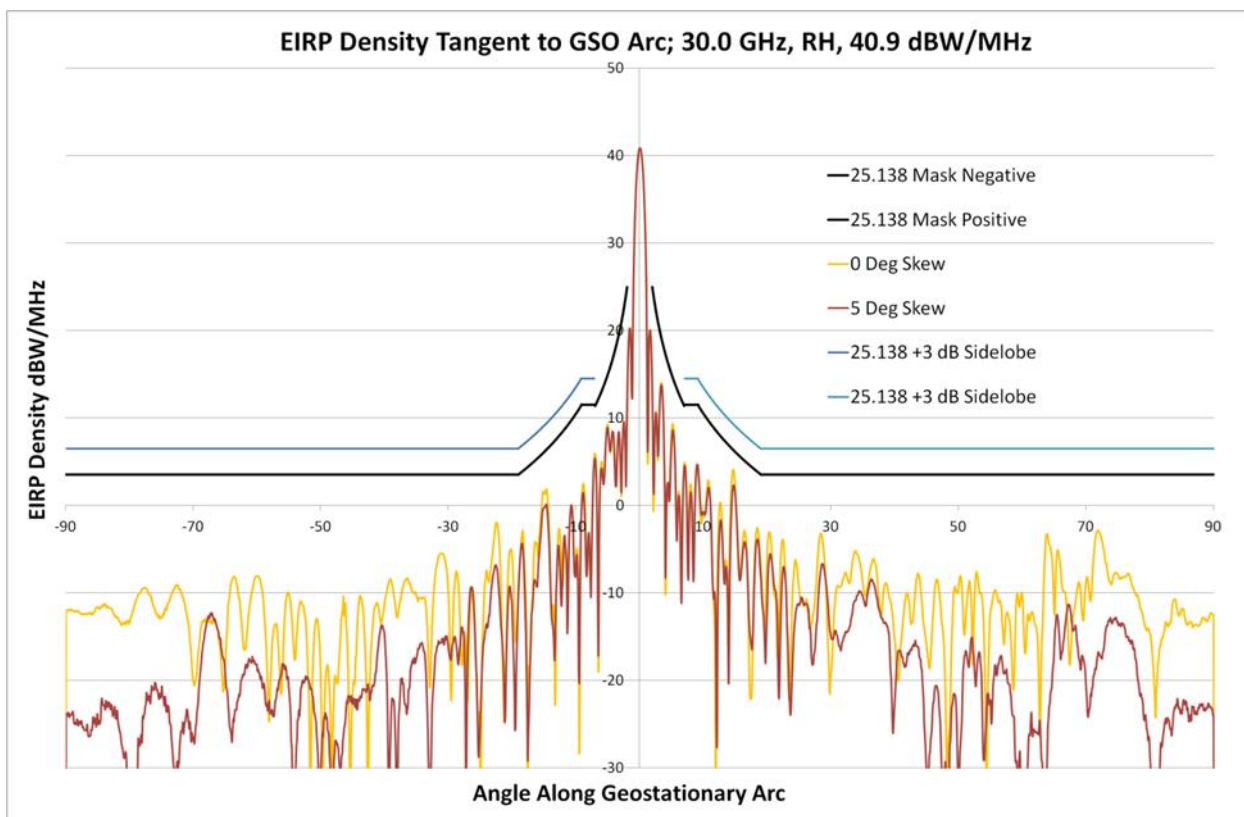
Figure 8 – EIRP Density tangent to GSO Arc, 30.0 GHz, RHP, 40.9 dBW/MHz, -90 to +90 deg., 25.138(a)(1) limits
