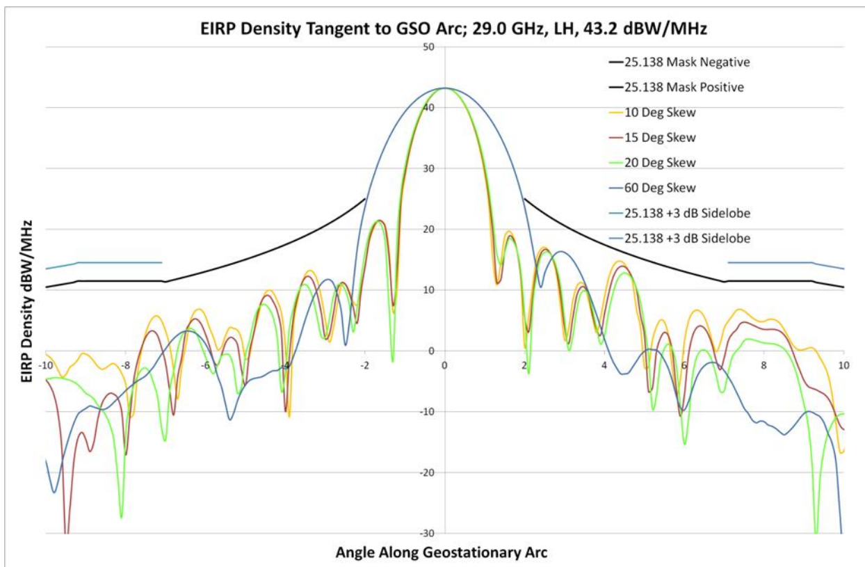
Figure 9 – EIRP Density tangent to GSO Arc, 29.0 GHz, LHP, 43.2 dBW/MHz, -10 to +10 deg., 25.138(a)(1) limits
