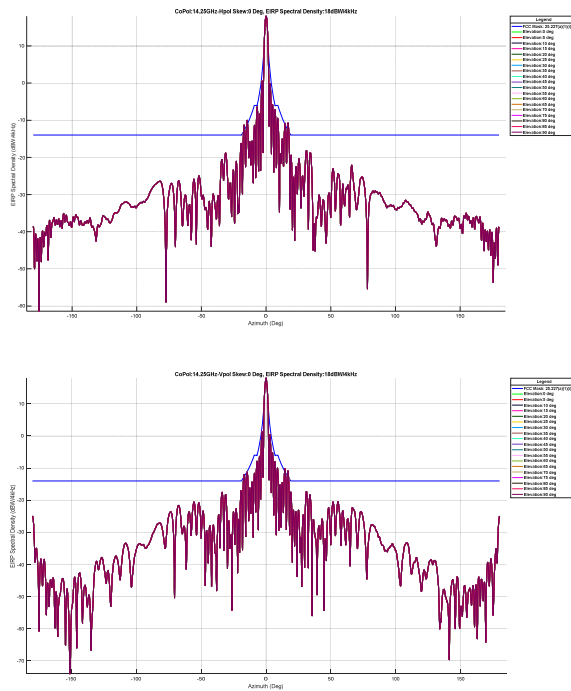
Figure 1 – EIRP Density for Horizontal and Vertical Polarization with 0^\circ Skew (and 0^\circ to 90^\circ elevation) at 14.25 GHz to Show 47 CFR Part 25.227(a)(1)(i)(A) compliance
